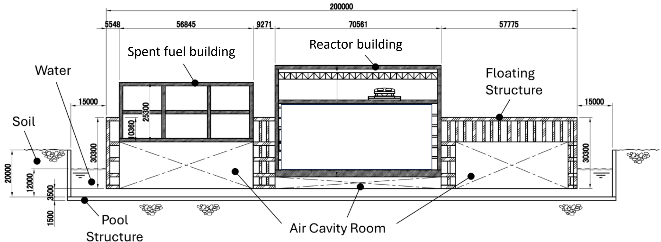
Cross-section view of the plant arrangement on the FSIS platform (numbers in the figure are in millimeters)
