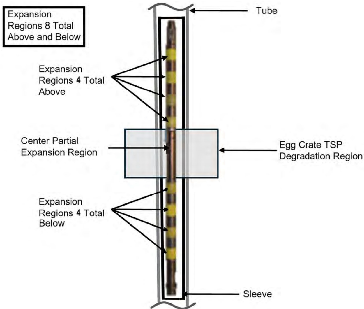
Figure 5-2: Typical Sleeve Installation
