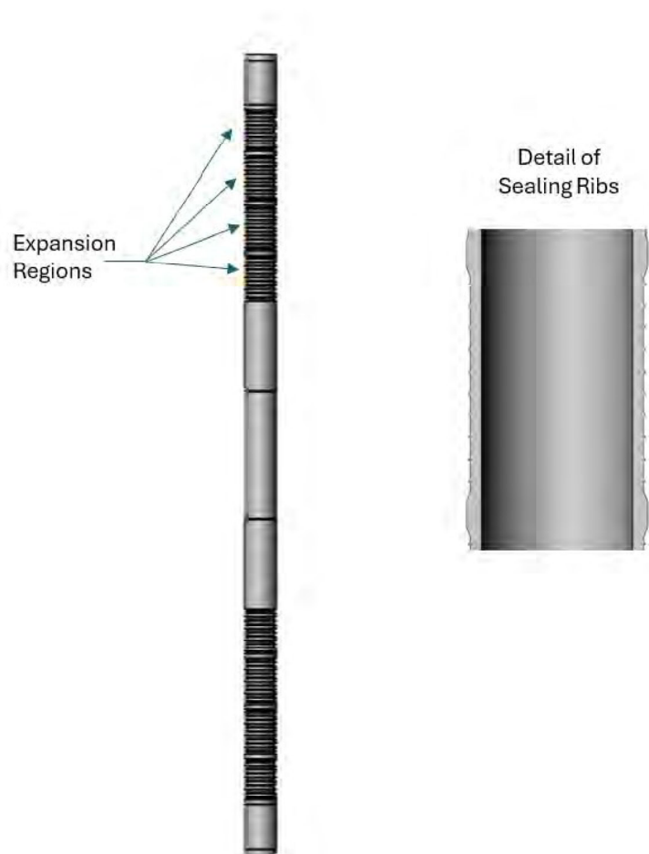
Figure 5-3: Mechanical TSP Sleeve
