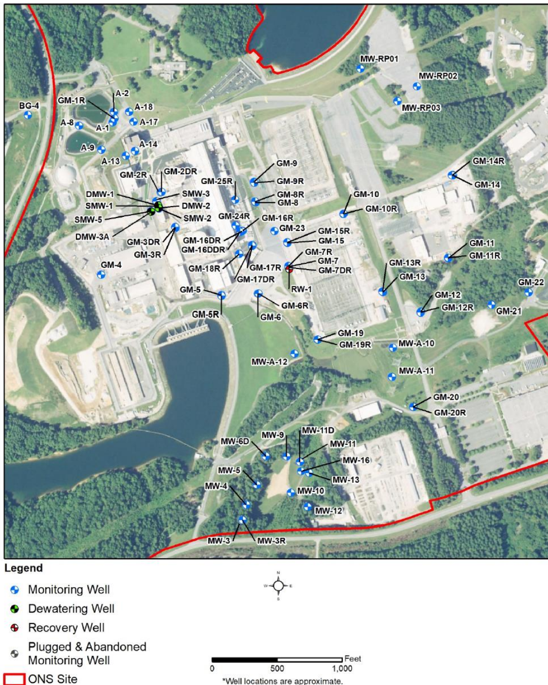
Figure 3-5 Oconee Station ONSite Groundwater Monitoring Wells. Source: Duke Energy 2021-TN8897.
