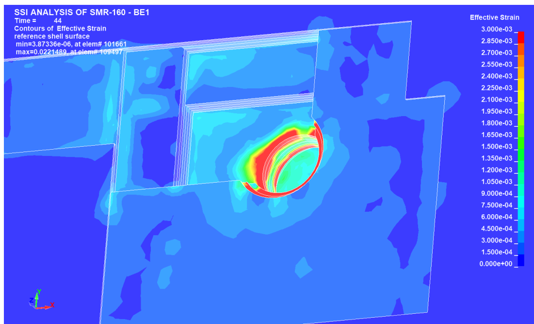
Figure 23. Soil strain distribution.
