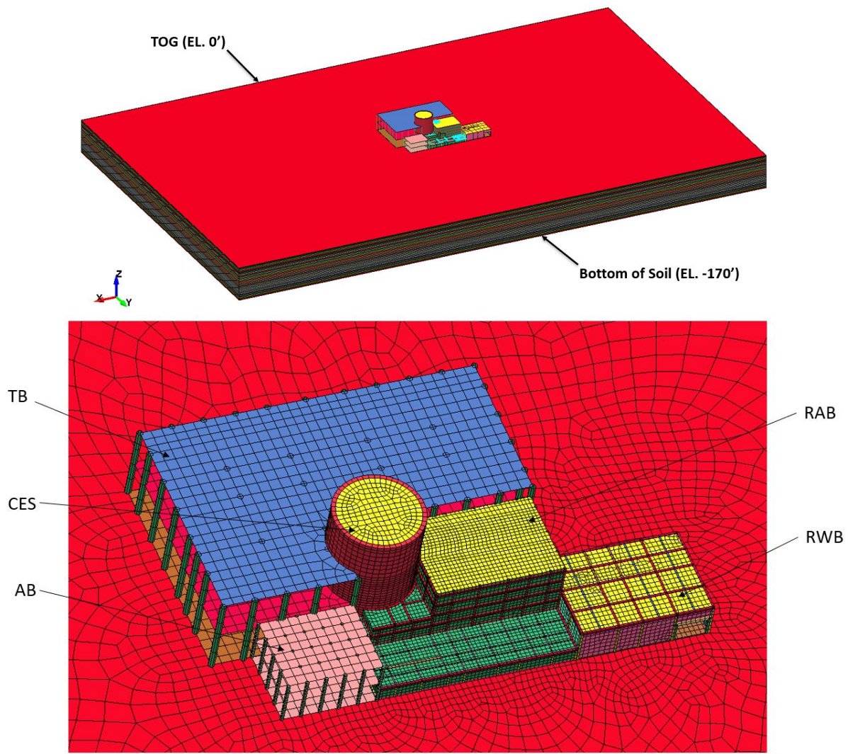
Figure 2. LS-DYNA model of overall SMR site.
