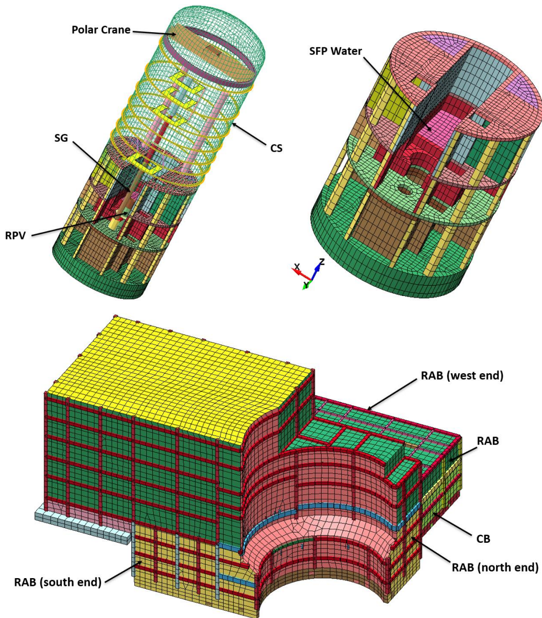
Figure 4. LS-DYNA model of CS and surrounding buildings.
