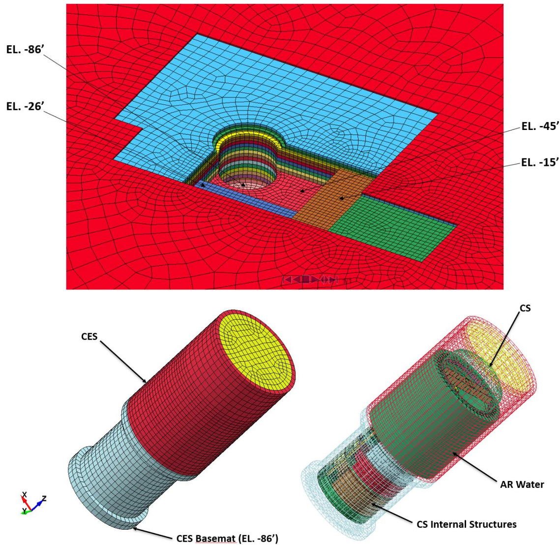
Figure 3. LS-DYNA model of SMR site, showing CES excavation, CES, and CS.
