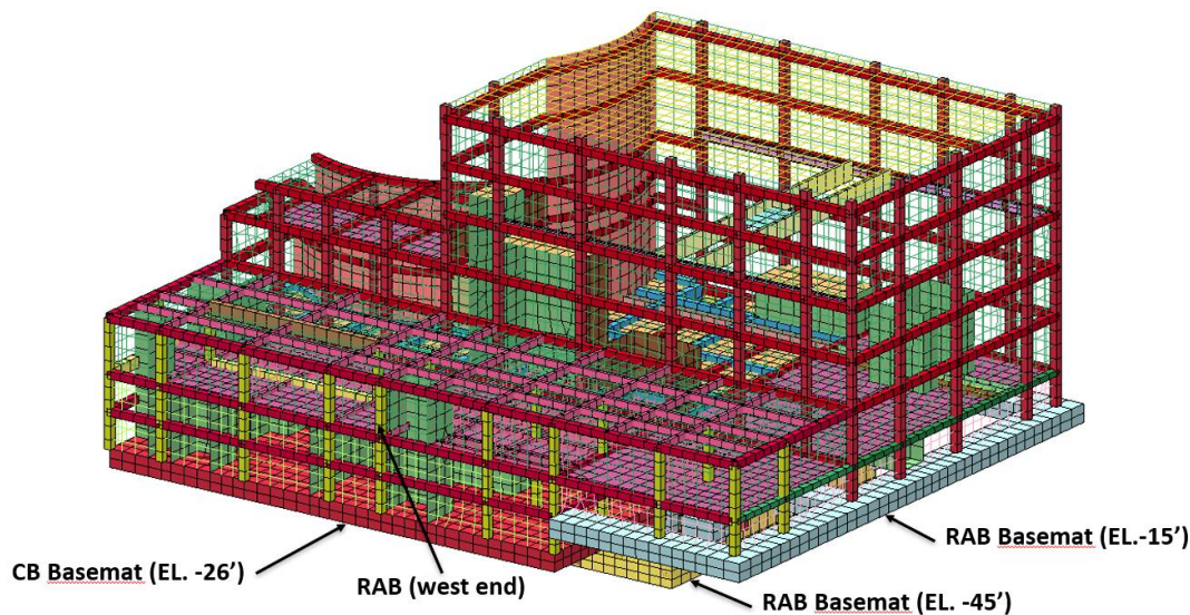
Figure 5. LS-DYNA model of RAB.
