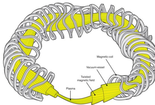
Stellarator
