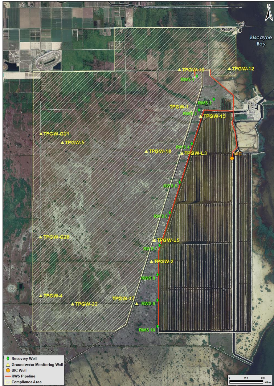
Figure 2-1 Compliance Area, RWS and Monitoring Wells West and North of the CCS (Source: FPL 2022d)
