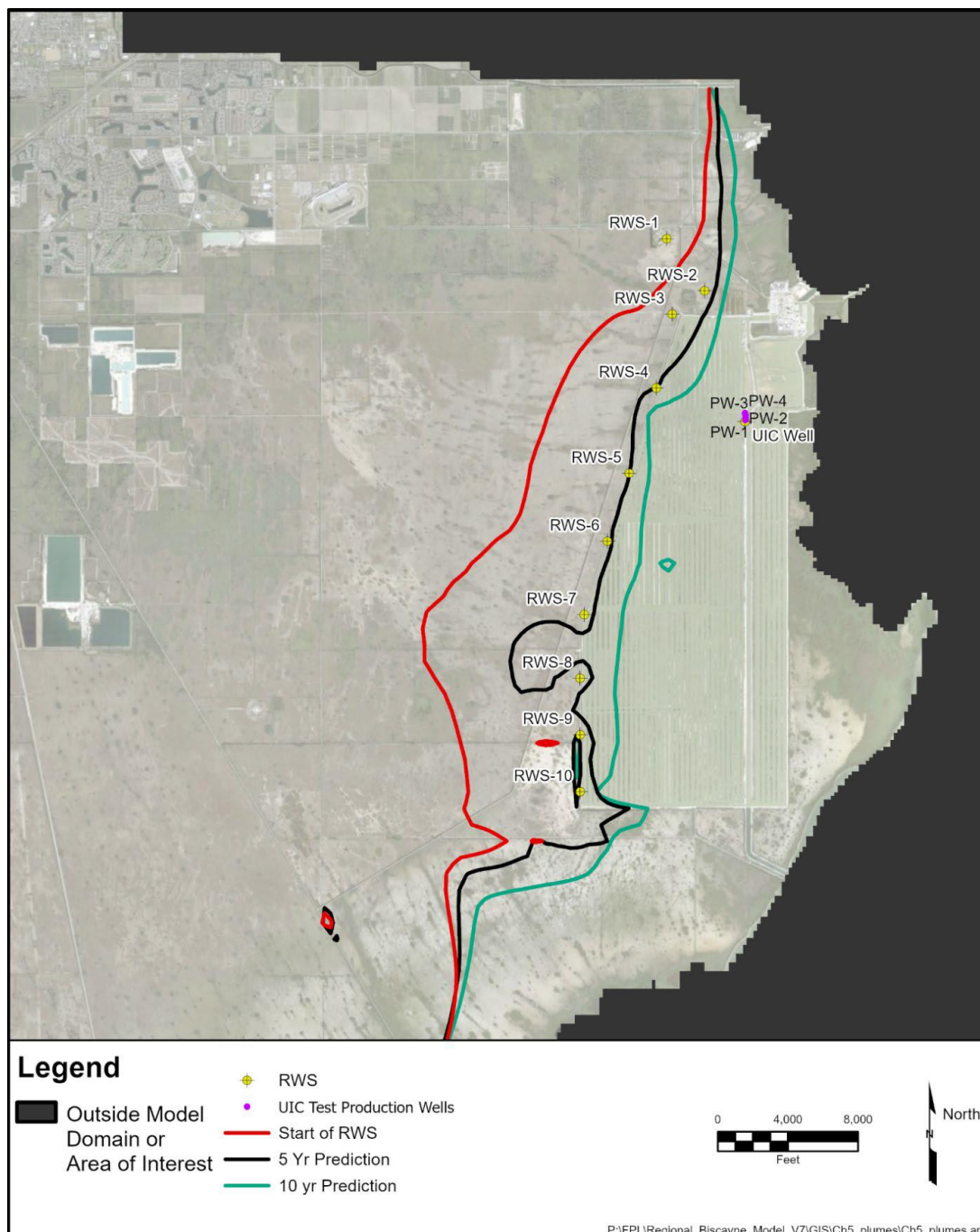
Figure 2-8 Location of the Initial, Year 5, and Year 10 Hypersaline Interface in Model Layer 9 (Source: FPL 2022d)
