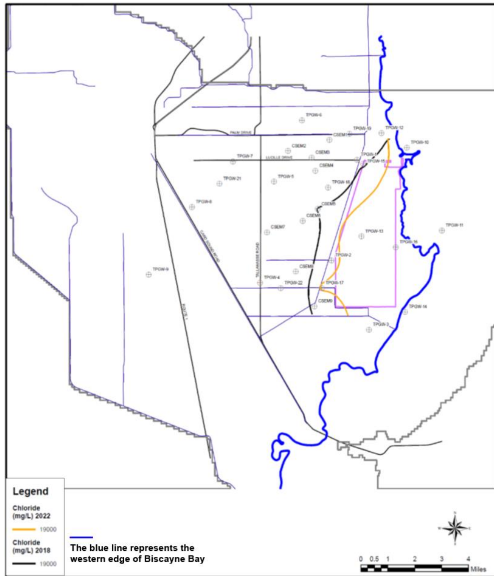
Figure 2-4 Comparison of the 2018 and 2022 Inland Extent of Hypersaline Groundwater (19,000 mg/L Chloride Isochlor) in the Shallow Horizon (Source: FPL 2022d)
