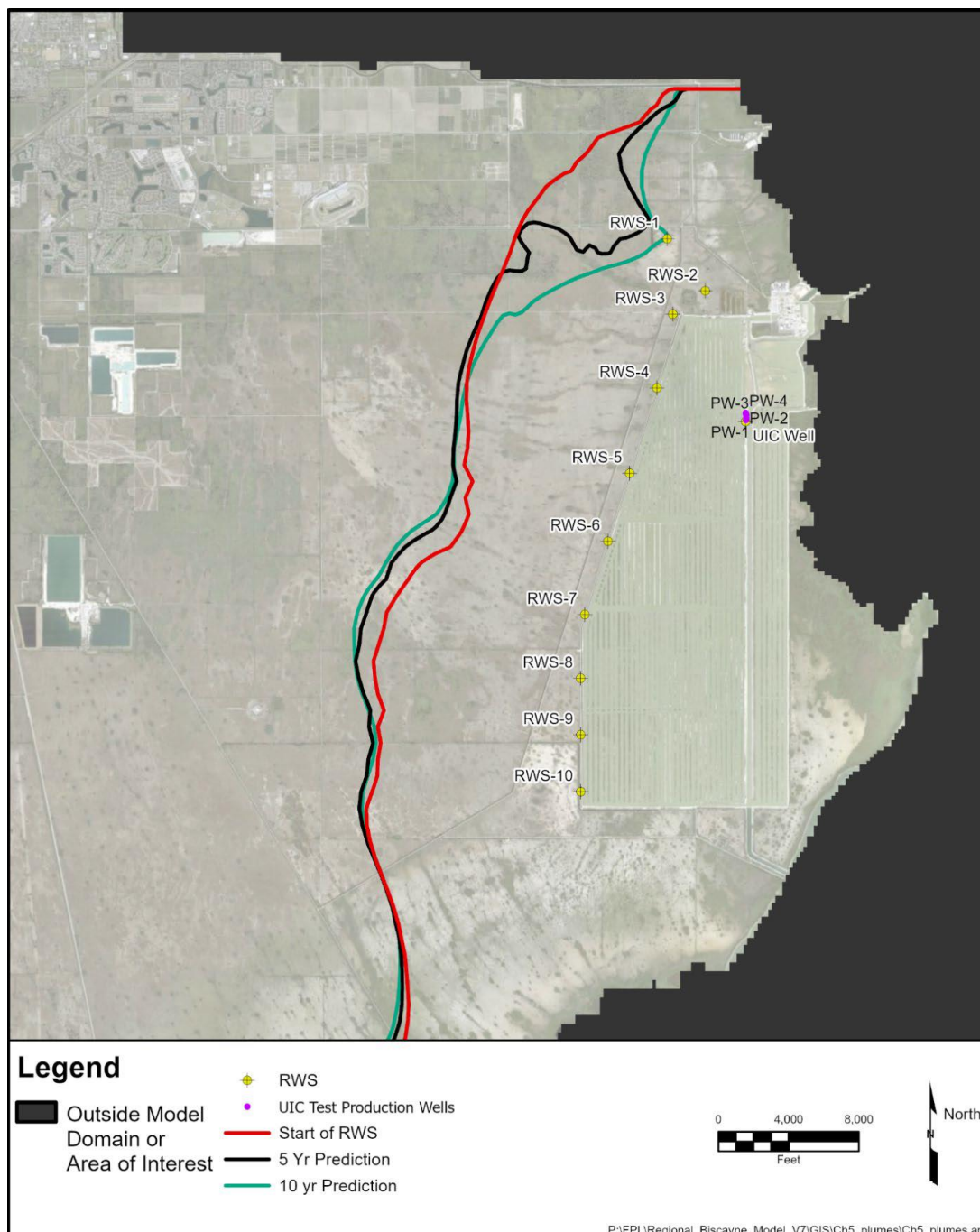
Figure 2-9 Location of the Initial, Year 5, and Year 10 Hypersaline Interface in Model Layer 16 (Source: FPL 2022d)
