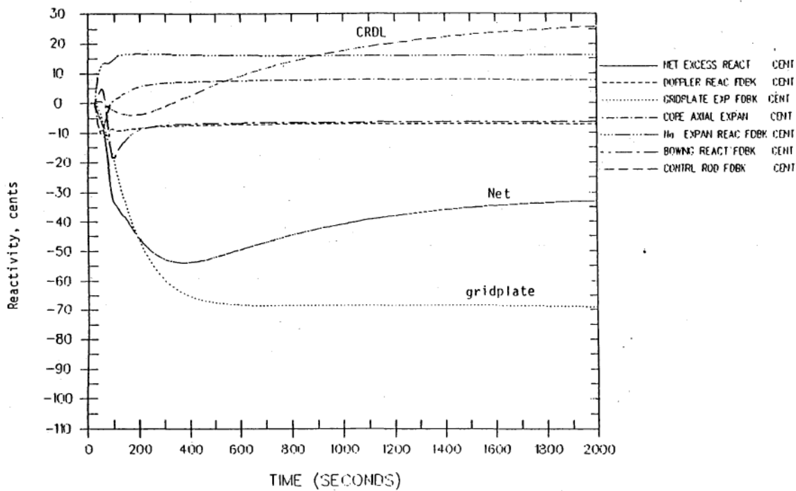
Figure 3.5.N-2. Reactivity
