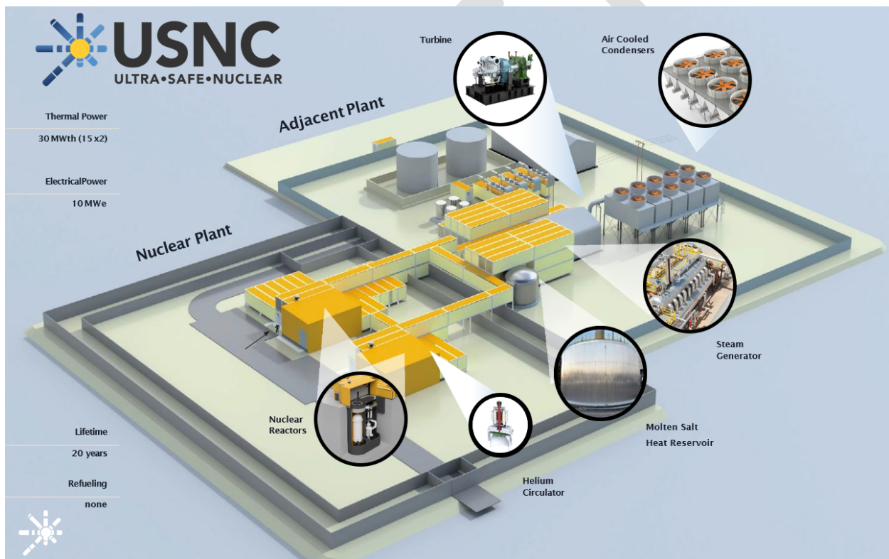
Exhibit 6-1: MMR™ Facility Layout displaying the Nuclear Plant (two micro-reactors) and an Adjacent Plant with molten salt heat storage
