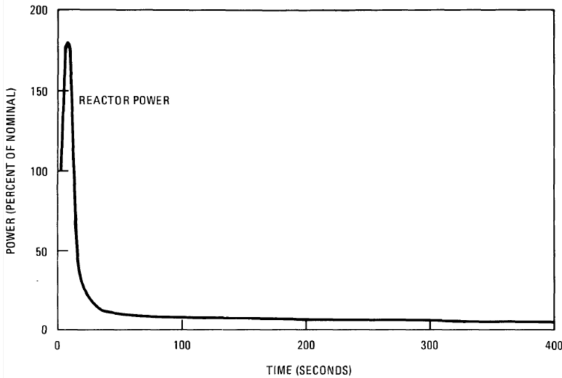
Figure 3.6.N-1. Reactor Power
