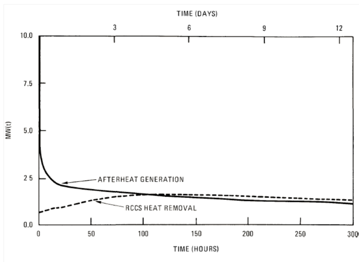
Figure 3.6.N-2. Heat Generation and Heat Removal
