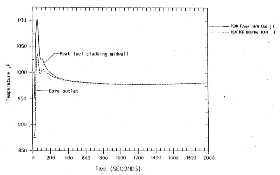
Figure 3.5.N-4. Peak Fuel-Cladding Midwall and Sodium Core Outlet Temperatures
