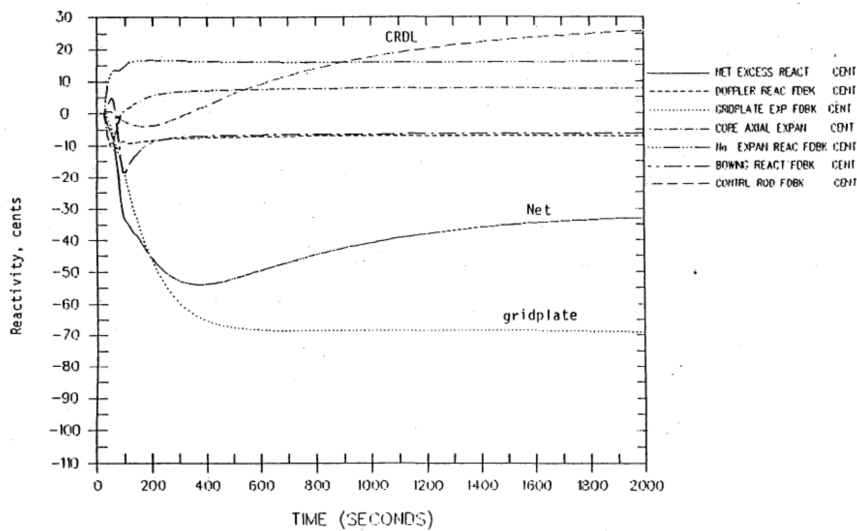
Figure 3.5.N-2. Reactivity
