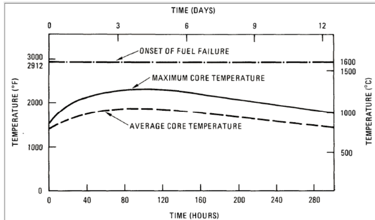
Figure 3.4.N-2. Core Temperature
