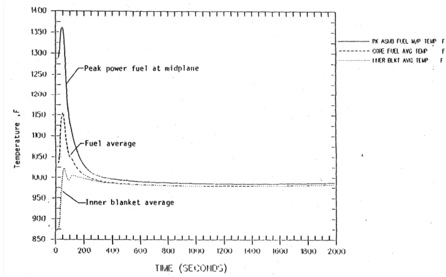
Figure 3.5.N-5. Fuel Temperatures
