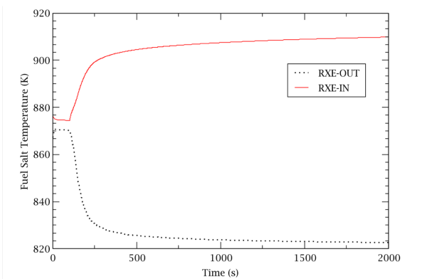
Figure 3.3.N-4. Fuel Salt Temperatures at the Outlet and Inlet of the Heat Exchanger
