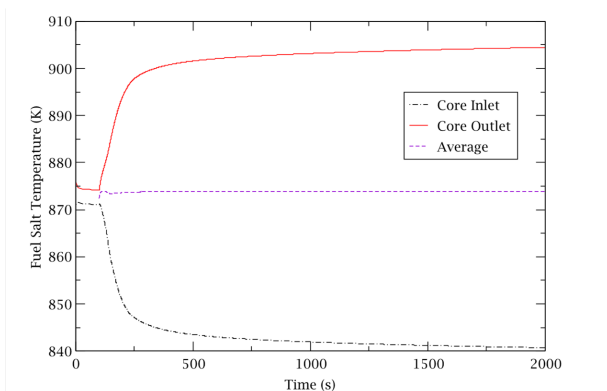
Figure 3.3.N-3. Fuel Salt Core Temperature
