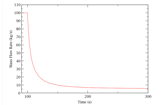
Figure 3.3.N-1. Fuel Salt Mass Flow Rate
