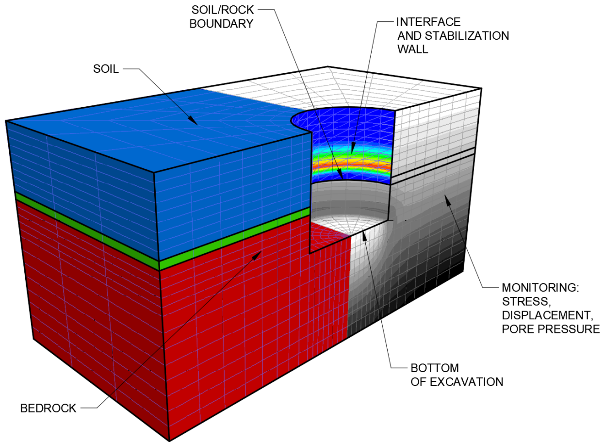
Figure 4-5: Excavation Modeling
