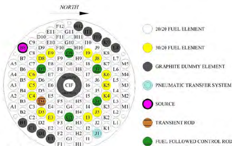
Figure 4.15 MNRC OCC
