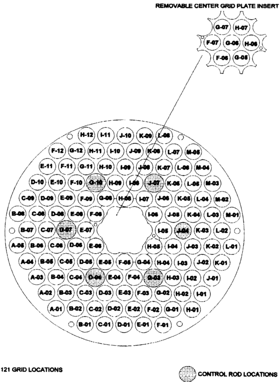
FIGURE 4.11 OPERATIONAL GRID NOMENCLATURE
