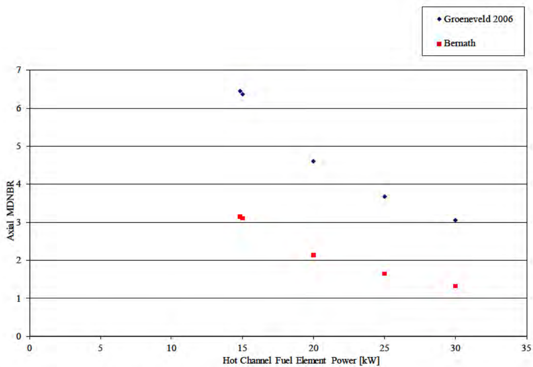
Figure 4.52 Hot channel MDNBR (OCC BOL core)
