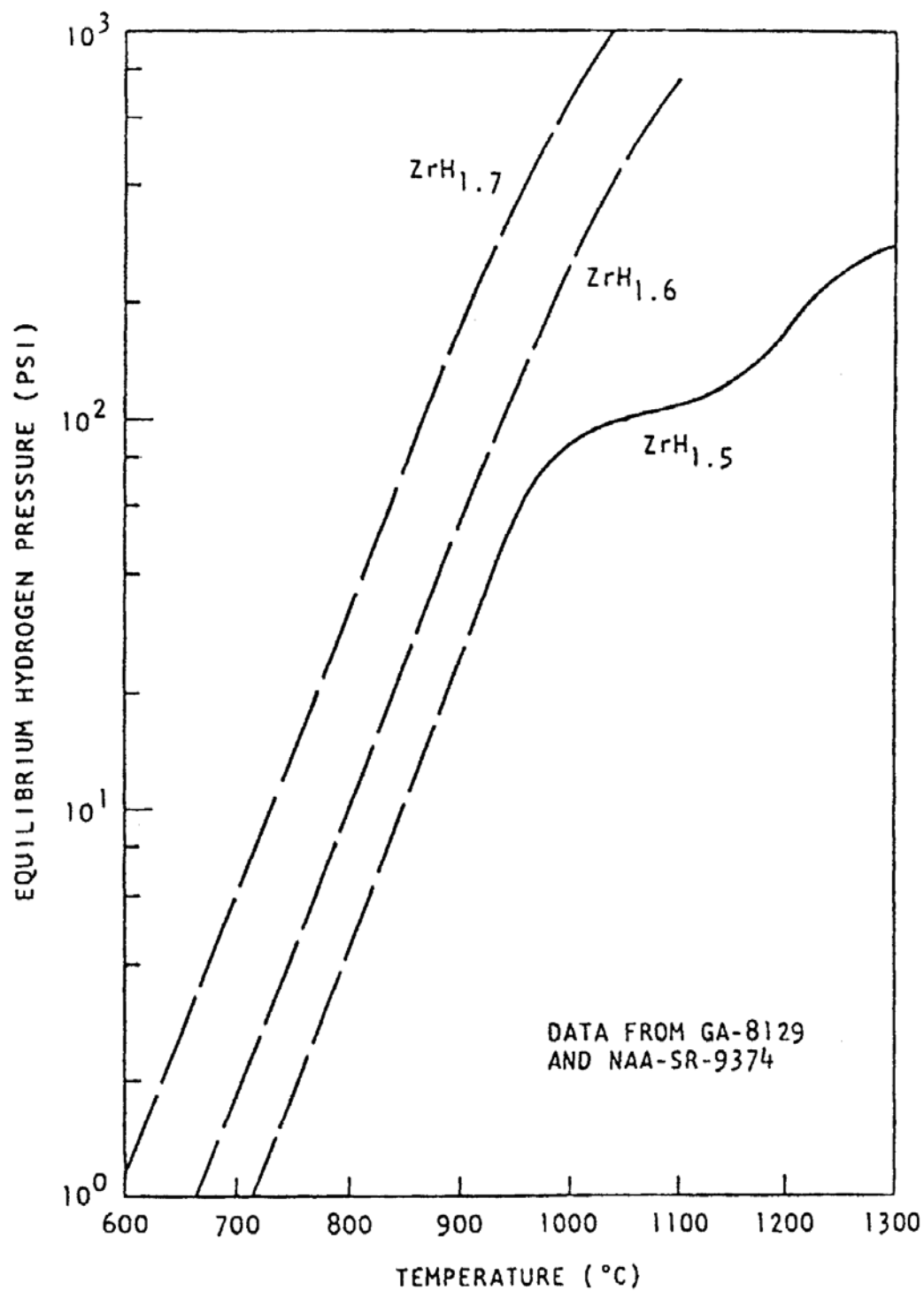
FIGURE 4.1 EQUILIBRIUM HYDROGEN PRESSURES OVER ZrH_x VERSUS TEMPERATURE
