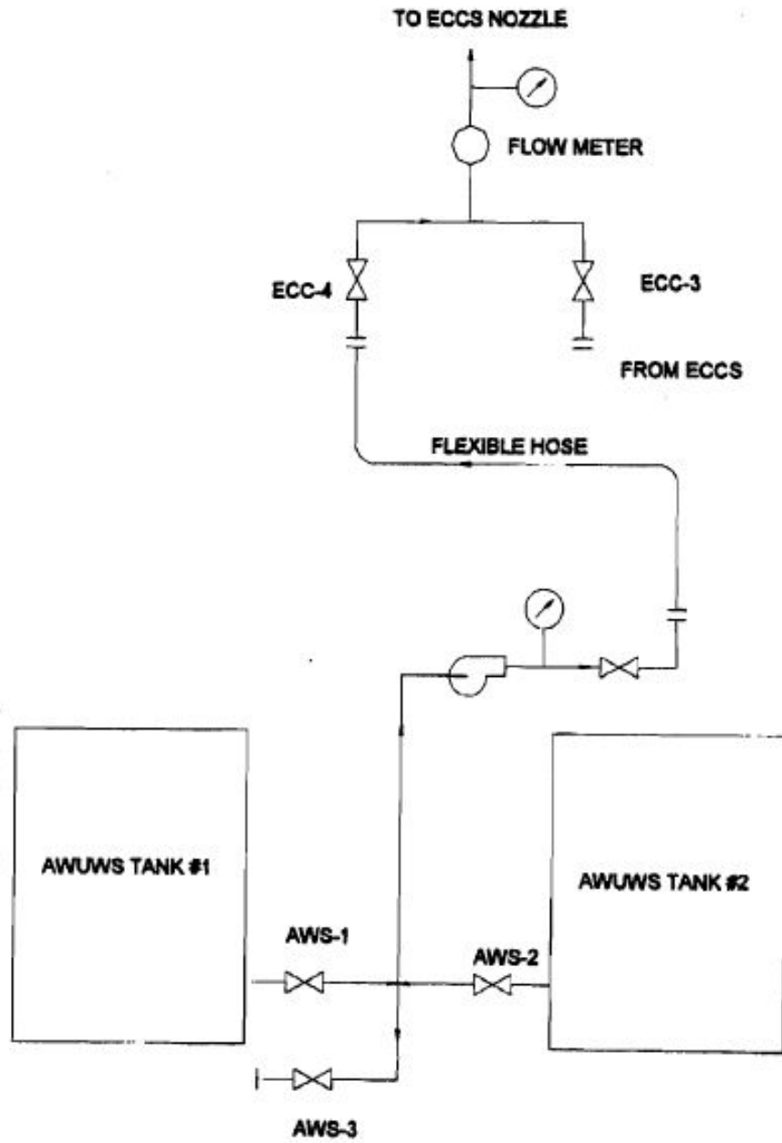
FIGURE 9.8 AUXILIARY MAKEUP WATER SYSTEM (AMUWS)
