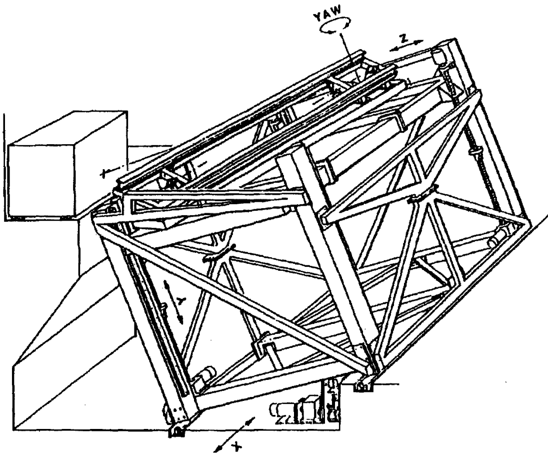
FIGURE 10.5 BAYS 1 AND 2 COMPONENT POSITIONING SYSTEM
