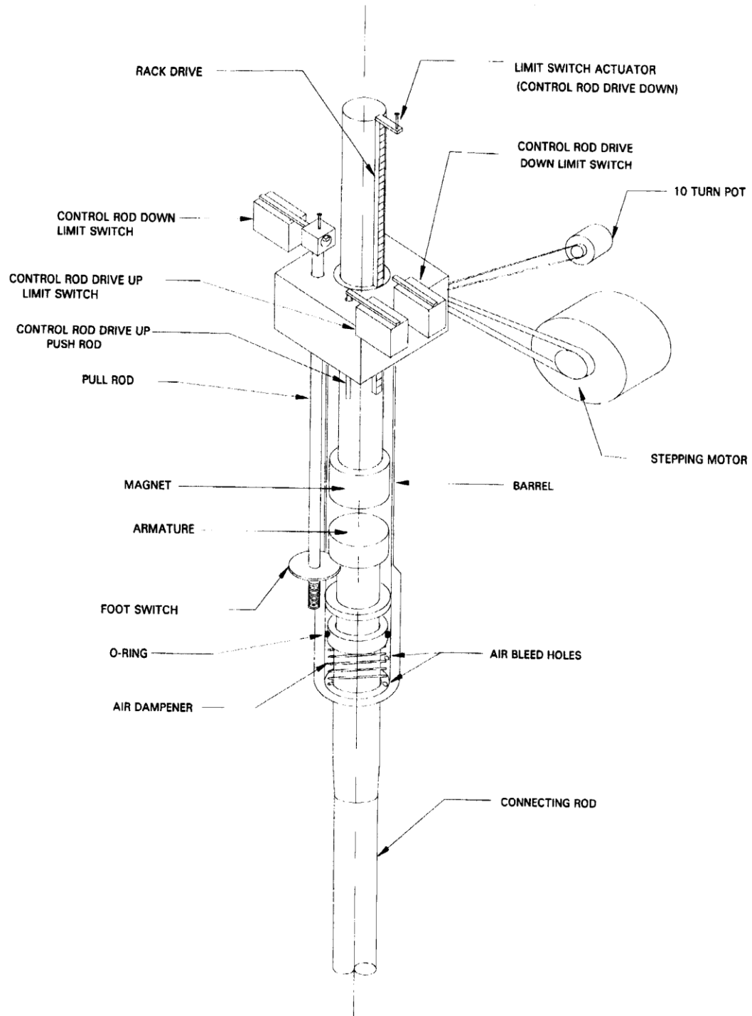
FIGURE 3.1 TYPICAL RACK-AND-PINION CONTROL-ROD-DRIVE MECHANISM
