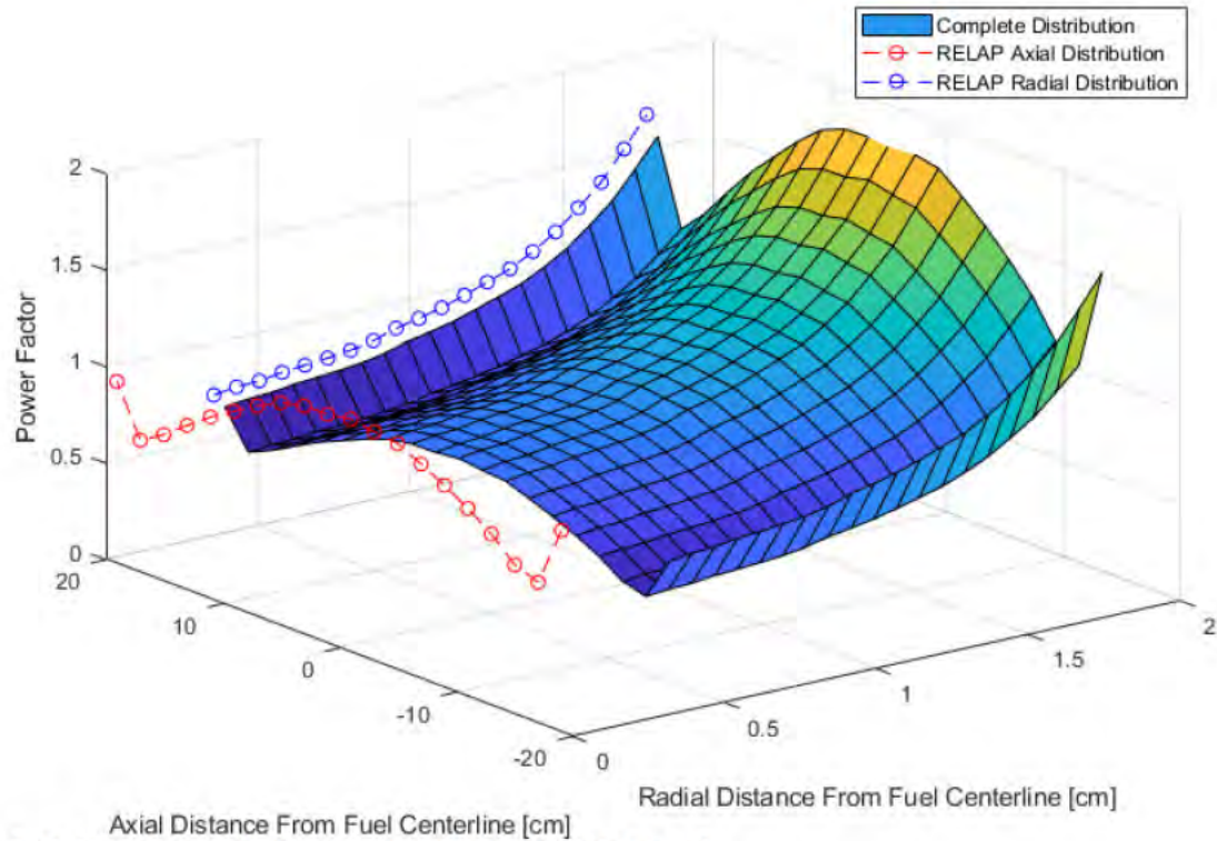
Figure 4.43: Hot element fuel power distribution (LCC-EOL Core)
