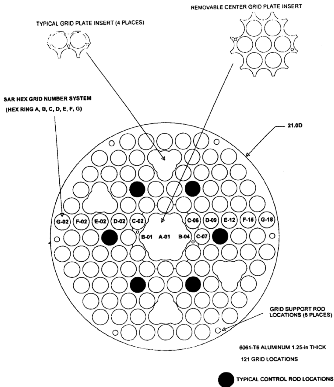
FIGURE 4.9 TOP GRID PLATE
