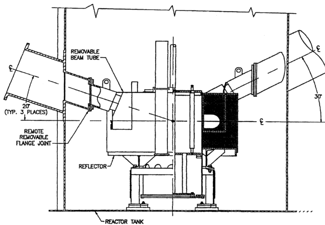
FIGURE 4.14 TYPICAL IN-TANK REACTOR CORE AND BEAM TUBE ASSEMBLY
