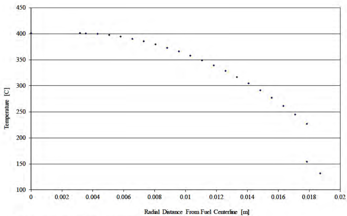
Figure 4.53: Radial temperature distribution at 14.81 kW th (OCC BOL Core)
