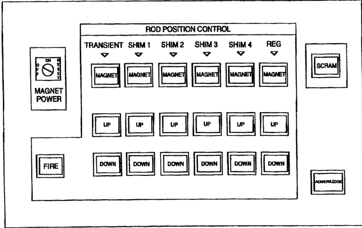
FIGURE 7.5 TYPICAL ROD CONTROL PANEL
