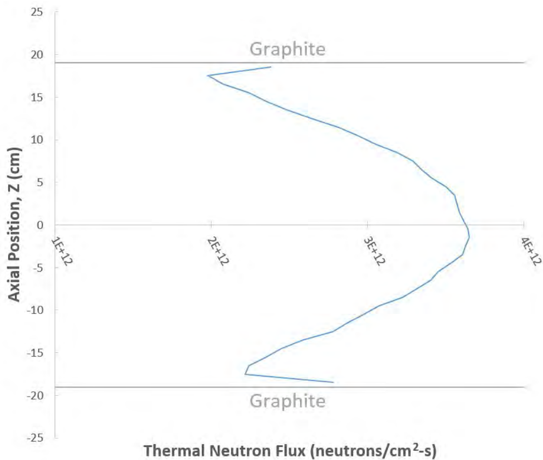
Figure 4.38 Axial thermal neutron flux distribution of the hot fuel rod at 16 location at 1.0 MW operating power. The length of the fuel meat, i.e. U-ZrH, is 15", or 38.1 cm.
