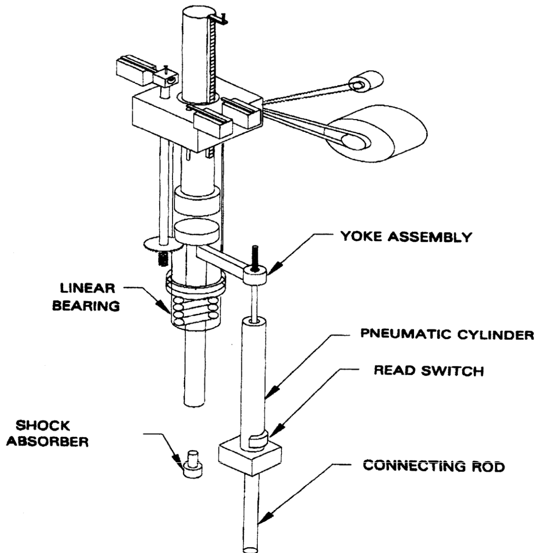
FIGURE 3.2 TYPICAL ADJUSTABLE FAST TRANSIENT ROD DRIVE
