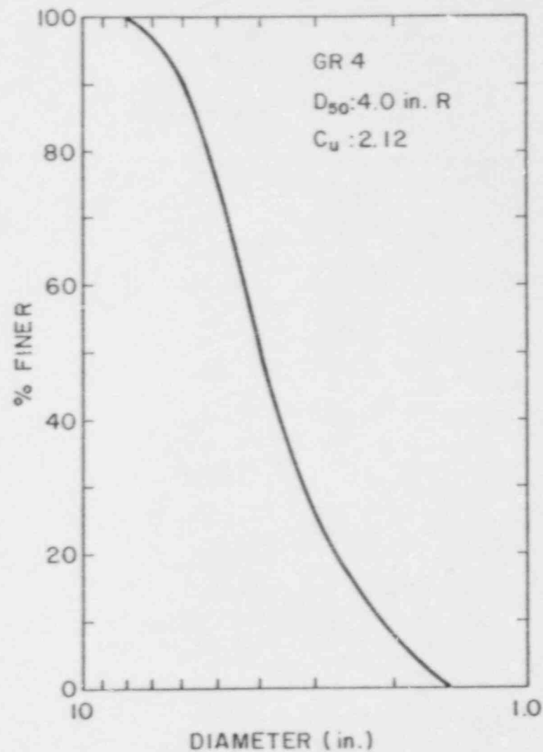
Figure A.4. Grain size distribution of grade 4 (GR4) riprap. D_{50} = median stone size, R = rounded shape, C_u = coefficient of uniformity.
