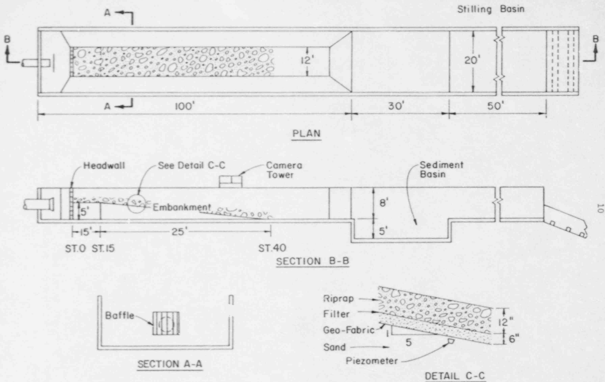
Figure 2.1. Outdoor flume schematic.
