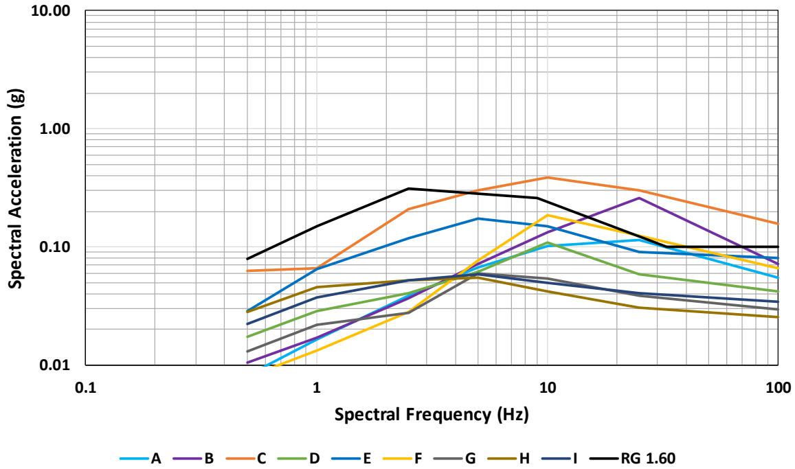
Figure 3-3 UHS for nine CEUS sites corresponding the 1 \times 10^{-3} exceedance frequency.
