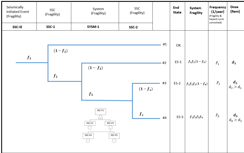
Figure 2-3 Schematic event and fault tree diagram showing seismic LBEs corresponding to an initiating event
