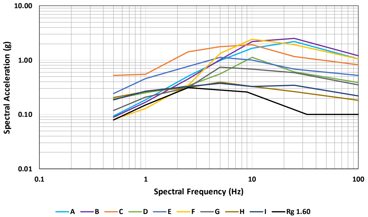
Figure 3-6 UHRS for nine CEUS sites corresponding the 1 \times 10^{-5} exceedance frequency
