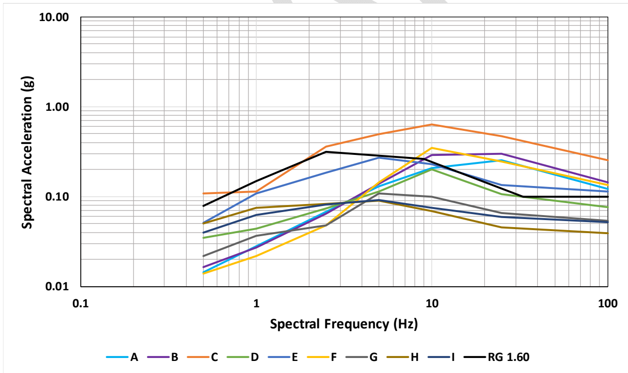
Figure 3-4 UHS for nine CEUS sites corresponding the 4 \times 10^{-4} exceedance frequency.
