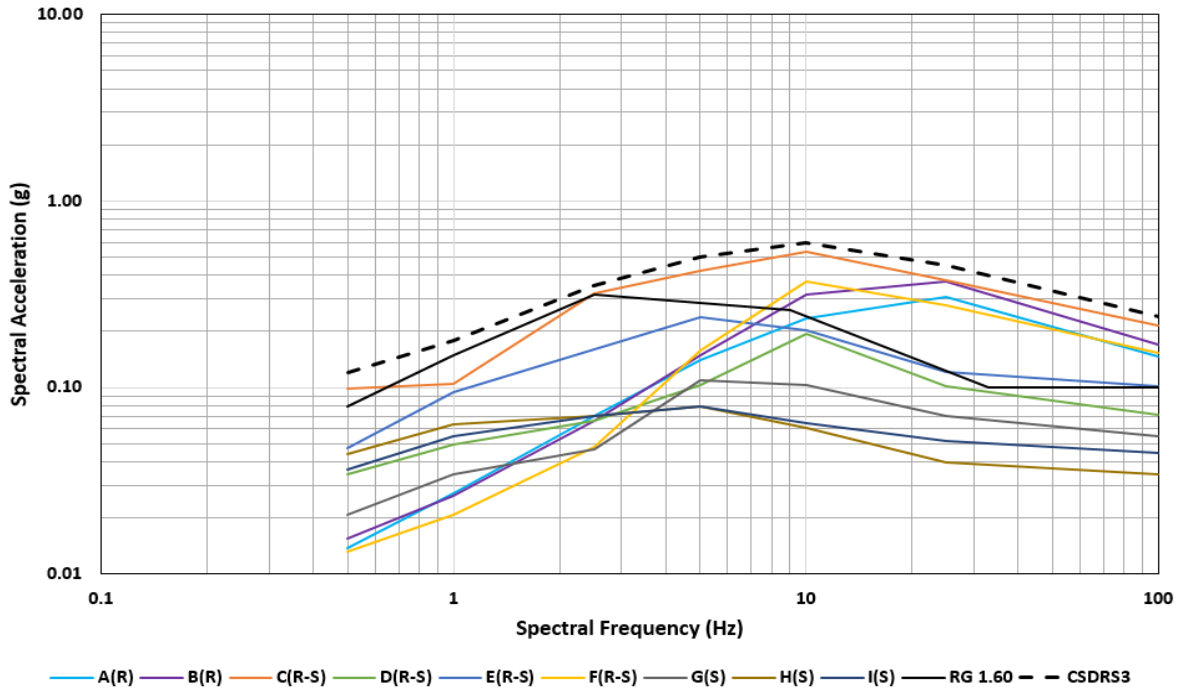
Figure 3-12 SSDRS-3 for all nine CEUS sites compared an RG-1.60 spectrum anchored at 0.1 g and the corresponding CSDRS
