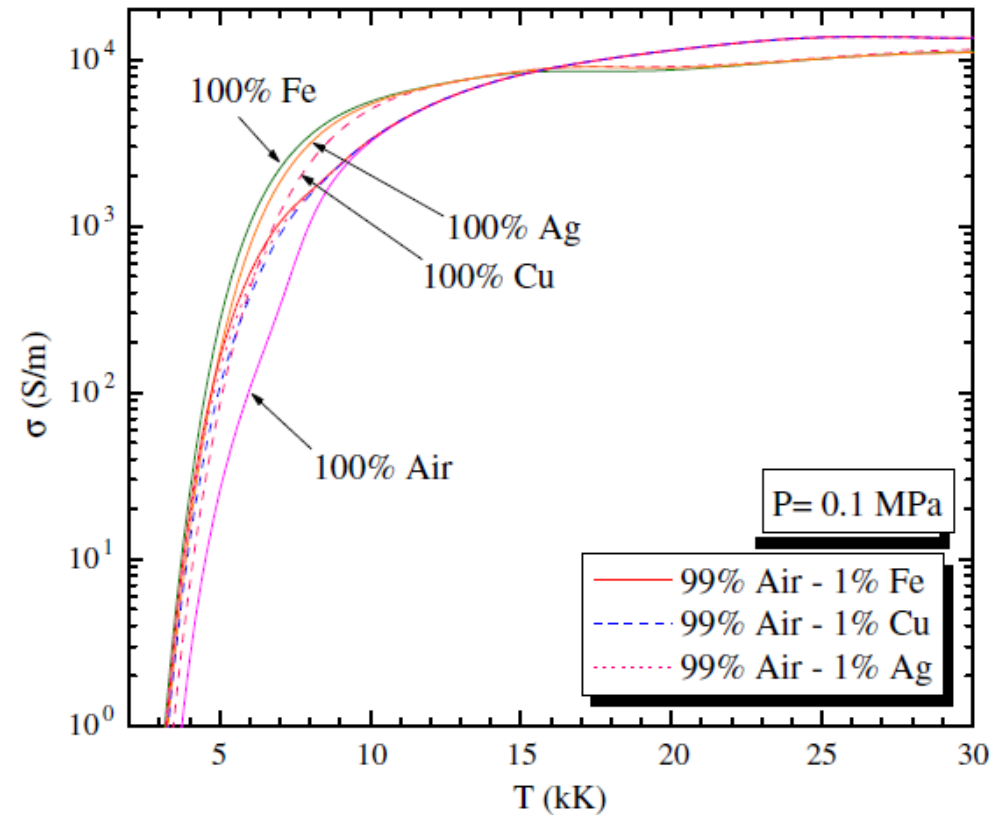
Influence of metallic vapours on the electrical conductivity.
