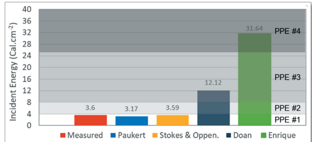
Figure 7 – Bar chart of incident energy measured and calculated using simplified models for a 1-MW PV system in inverter level and respective PPE categories according to NFPA 70E-2018
