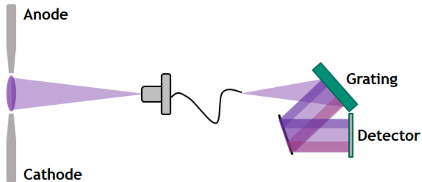
Optical emission spectroscopy
