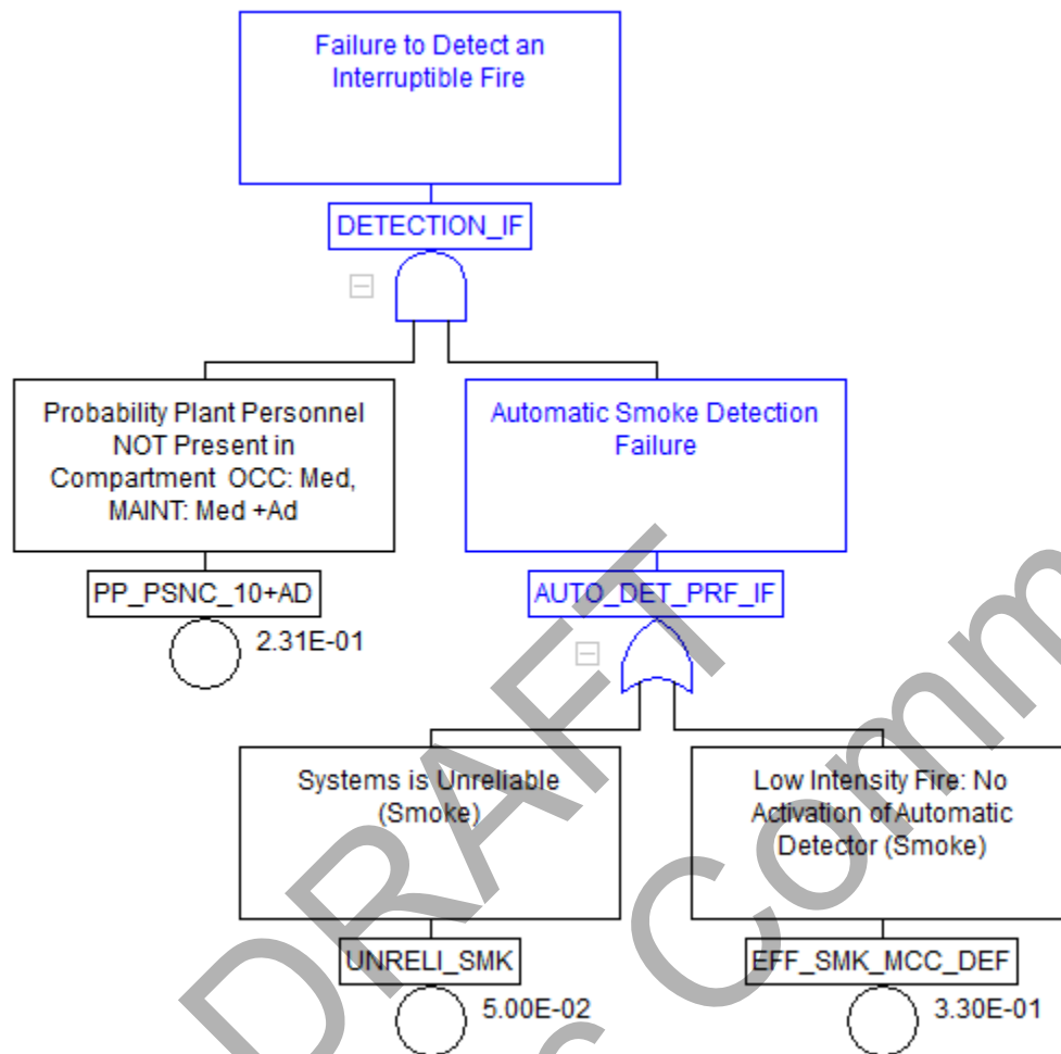
Figure 6-2 First Detection – Interruptible, NUREG/CR-6850 Appendix P Example
