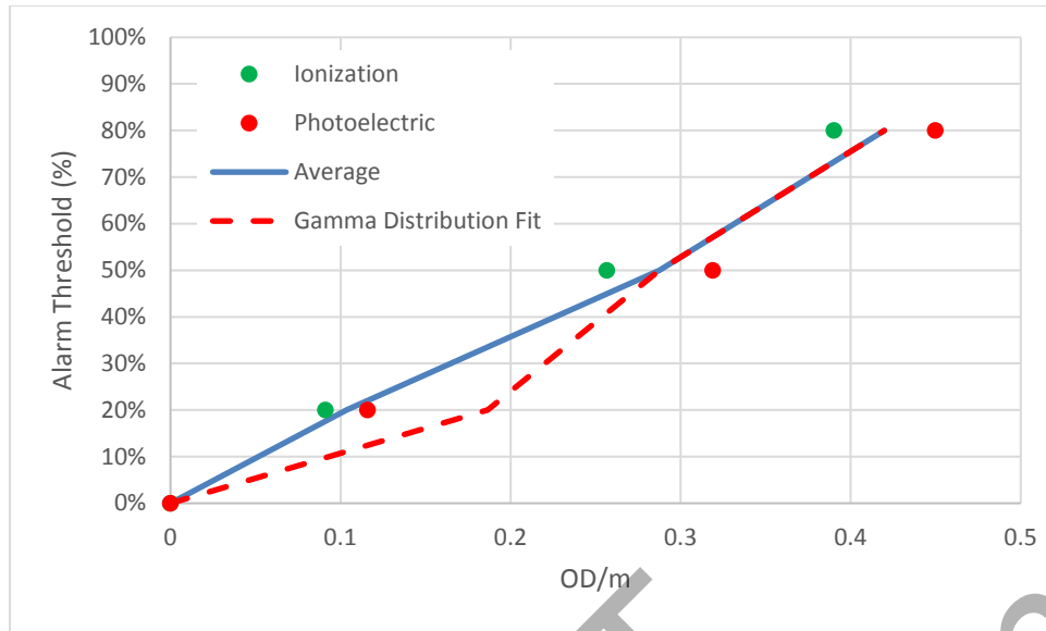
Figure B-1 Alarm Threshold Optical Density Gamma Distribution Fit
