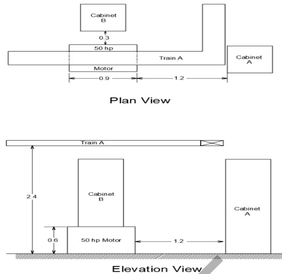
Figure 5-23 Motor Walkdown Distances
