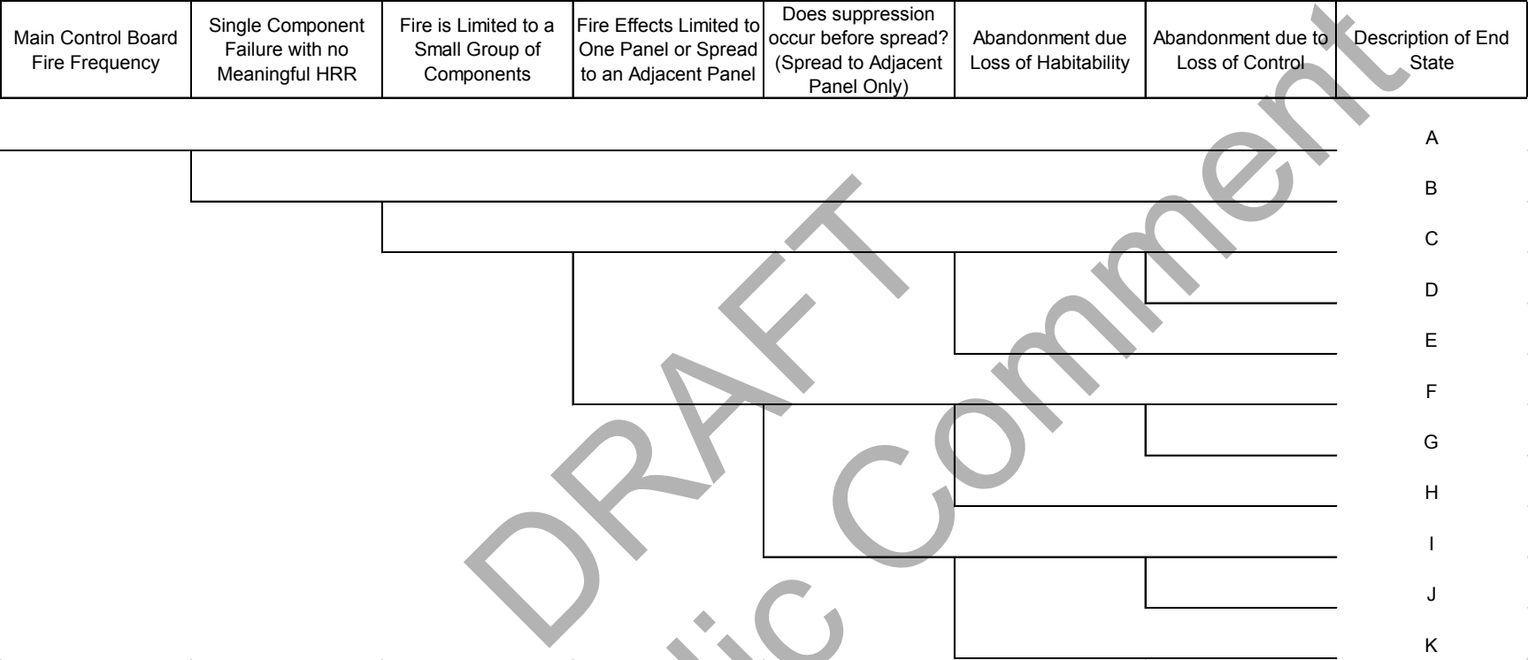
Figure 8-1 Main Control Board Fire Event Tree
