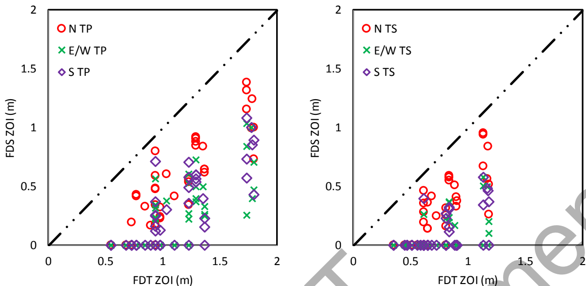
Figure 2-20 FDS Predicted Cabinet ZOI vs. Unadjusted FDT s Predicted Open Fire ZOI for all Closed Cabinet Simulations (Left: Thermoplastic Results, Right: Thermoset Results)
