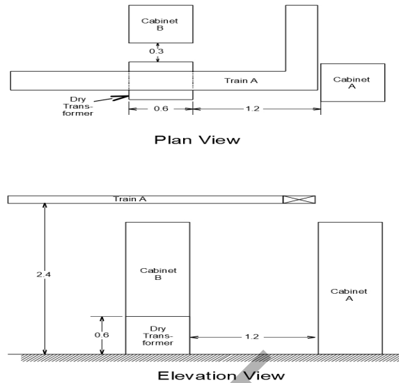
Figure 5-24 Transformer Walkdown Distances
