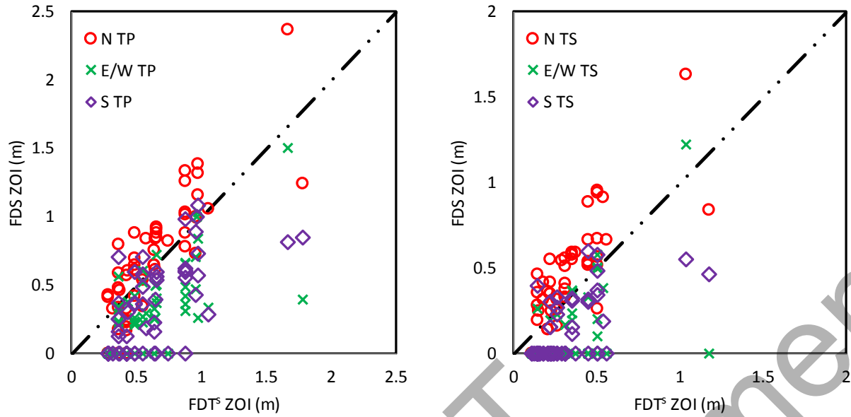
Figure 2-19 FDS Predicted Cabinet ZOI vs. Adjusted FDT s Predicted Open Fire ZOI for all Simulations (Left: Thermoplastic results, Right: Thermoset Results)
