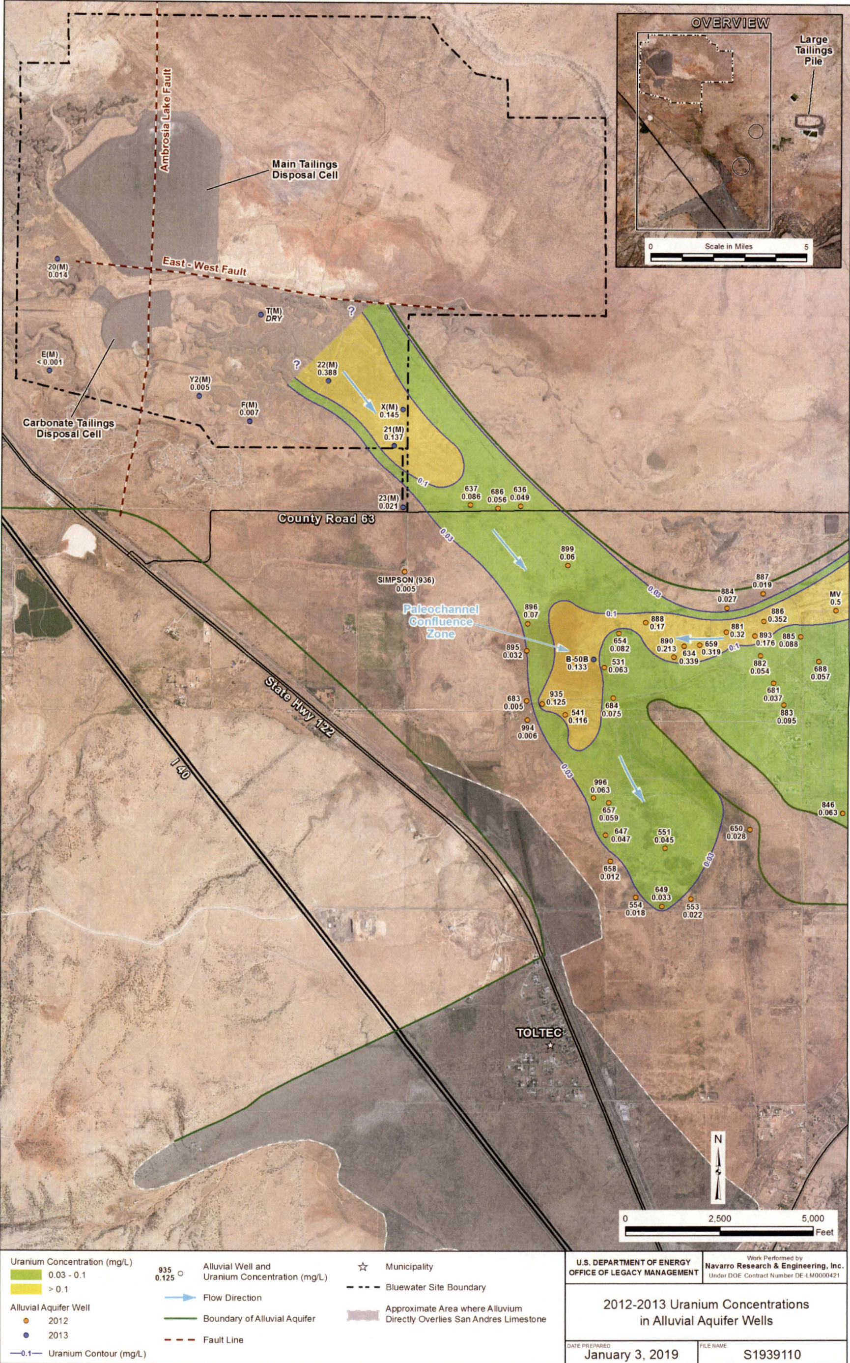
Figure 18. The 2013 Uranium Plume Map for the Alluvial Aquifer Based on Water Samples Collected in 2012 and 2013
