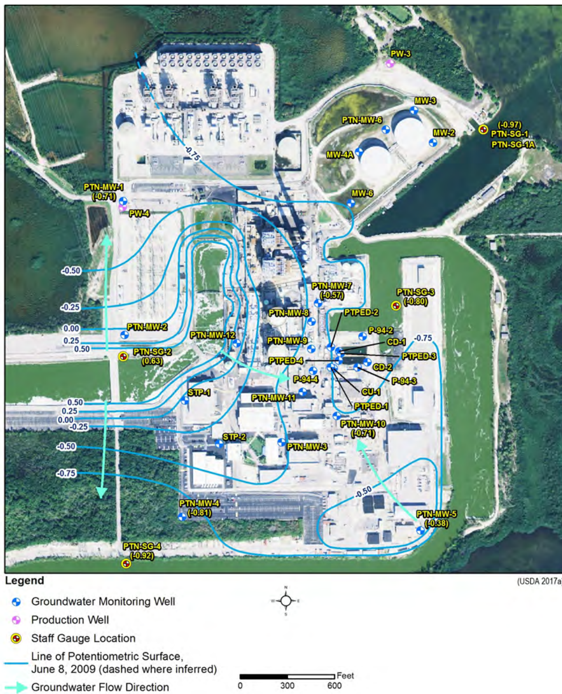
Figure 3.6-6 Turkey Point Potentiometric Surface Map Low Tide Intermediate Groundwater Elevation
