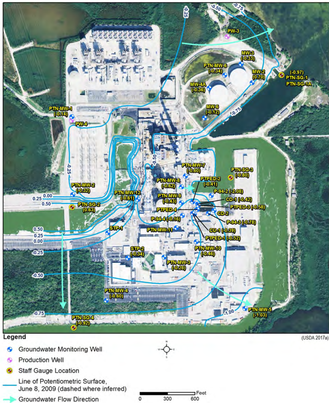
Figure 3.6-4 Turkey Point Potentiometric Surface Map Low Tide Shallow Groundwater Elevation
