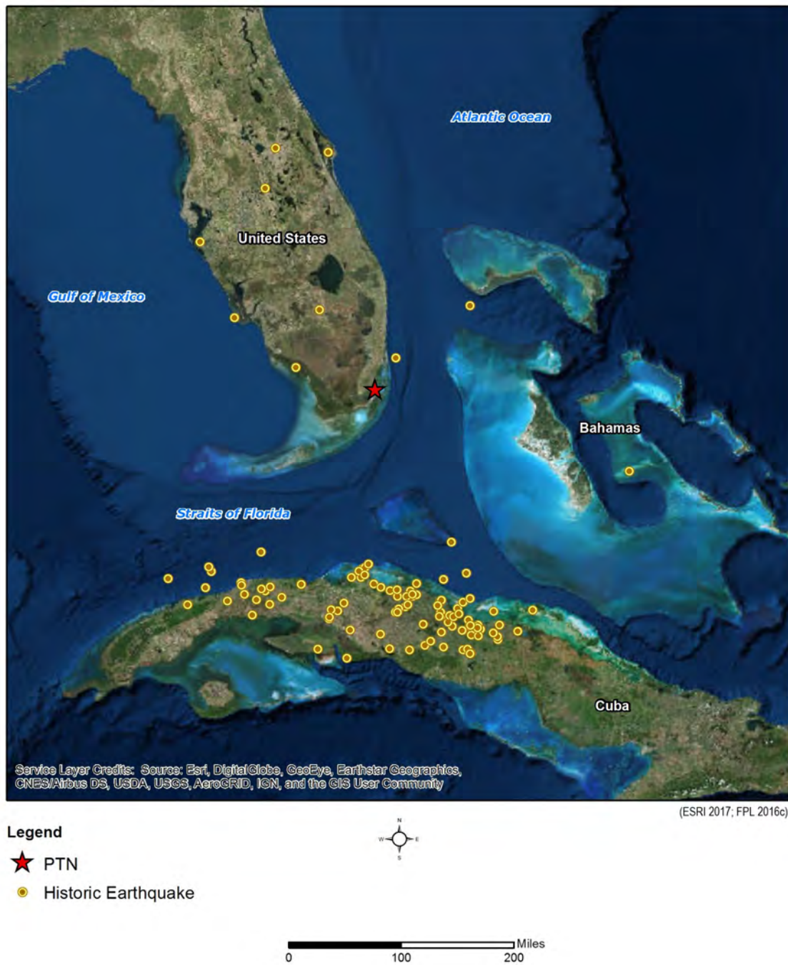
Figure 3.5-5 Historic Earthquakes
