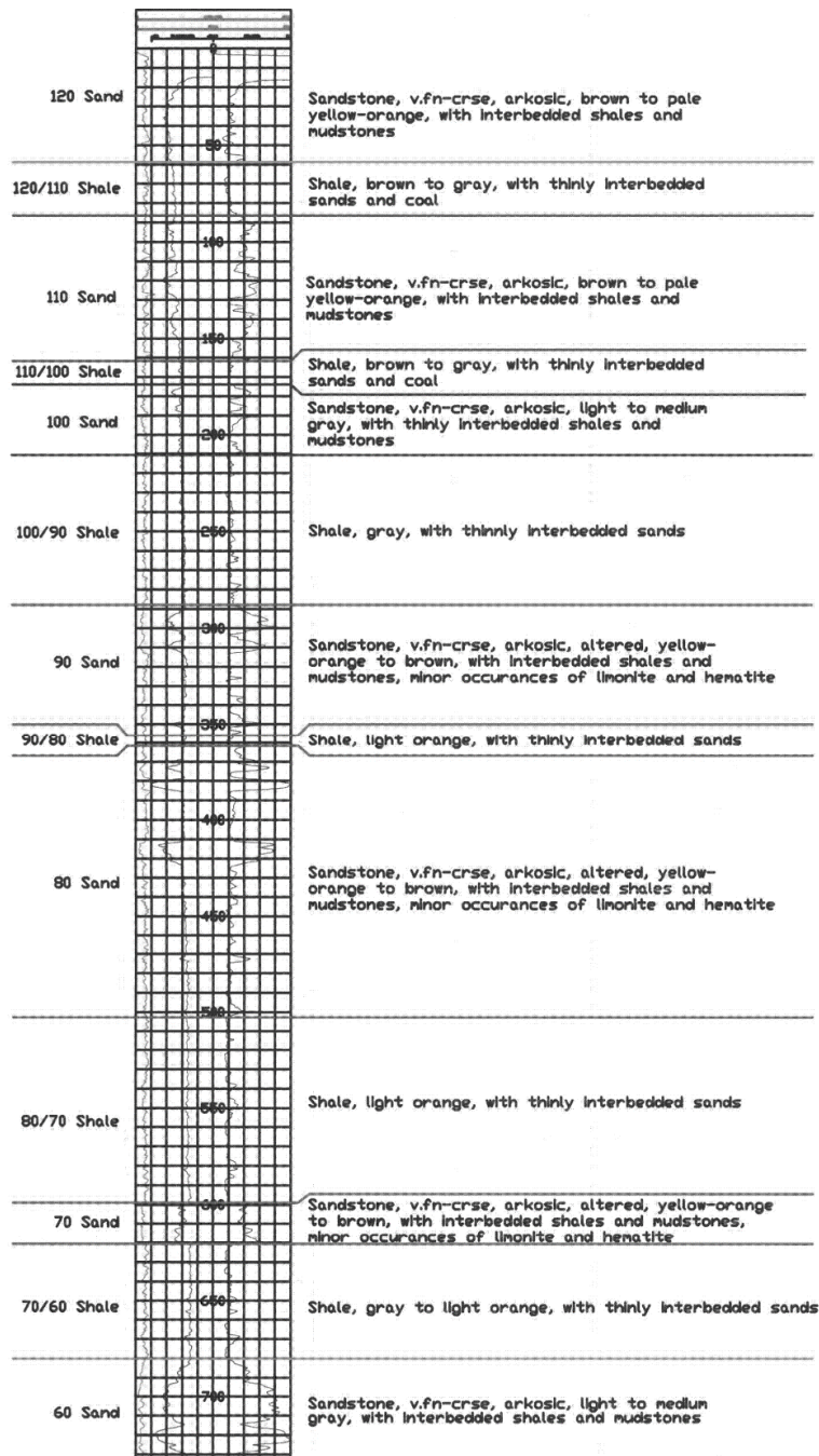
Figure 2.3-2 Type Log for Ludeman Project Stratigraphy
