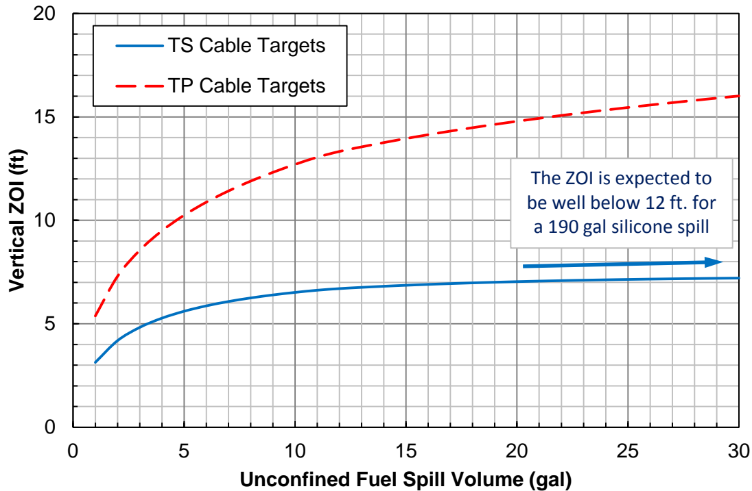
Figure 5.2.6 – Vertical ZOI for an Unconfined Silicone Liquid Spill Fire and a TS Target.
