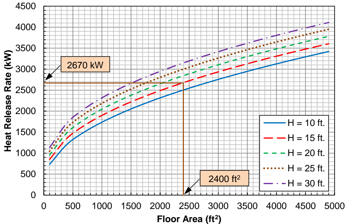
Figure 5.2.7 – Minimum HRR Required Creating a Damaging HGL for TS Targets in a Compartment with a Floor Area of 2400 ft² and Ceiling Height of 15 ft.
