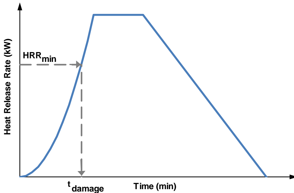
Figure 6.2.4 – Damage Time Determination for FDS1 Scenarios.
