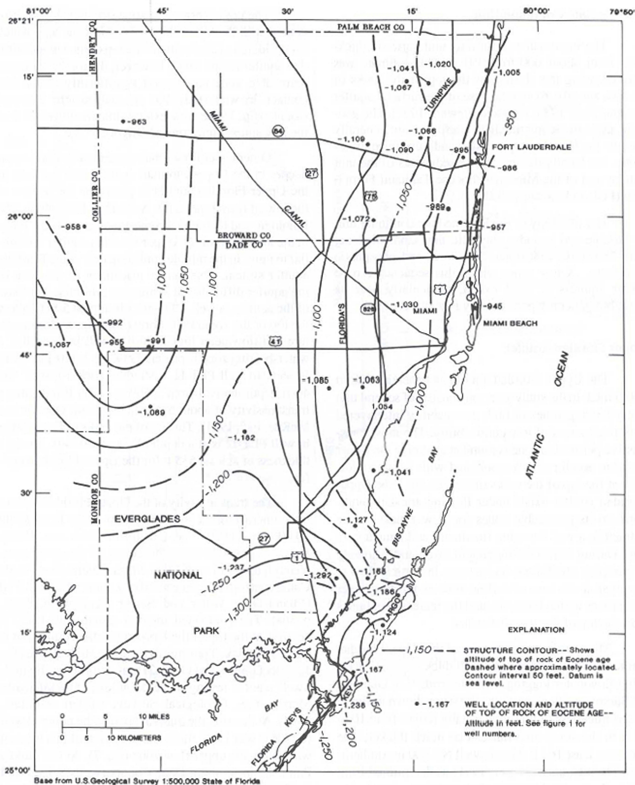
Figure 6. Altitude of the top of the rocks of Eocene age in southeastern Florida.
