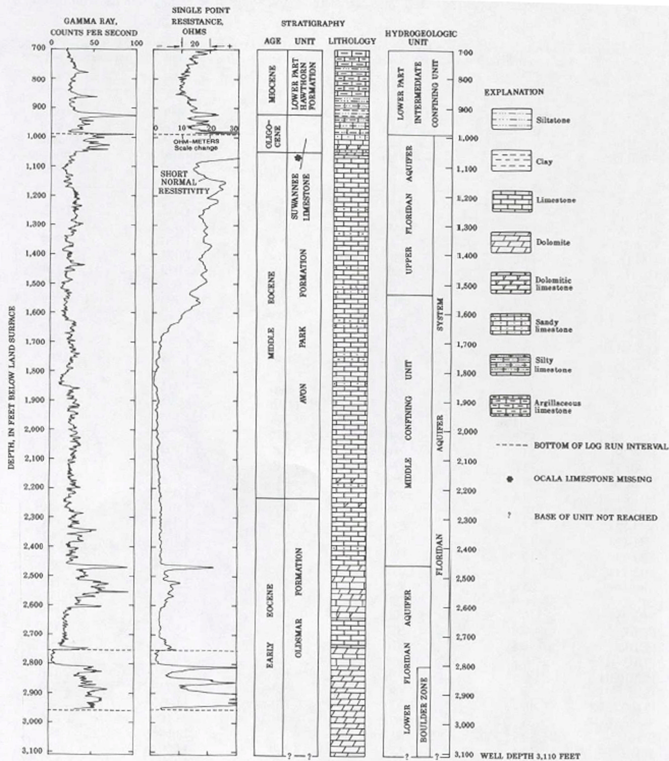
Figure 2. Selected geophysical logs, stratigraphy, and hydrogeologic units for well MDS-BZ1 near Biscayne Bay in southeastern Dade County.
