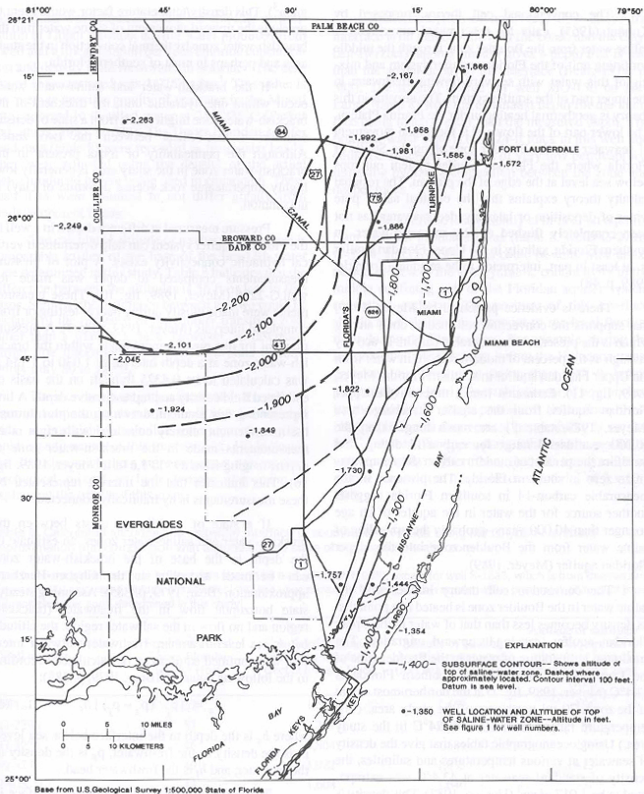
Figure 18. Altitude of the top of the saline-water zone in southeastern Florida. Method used to determine this altitude in each well is given in table 7.
