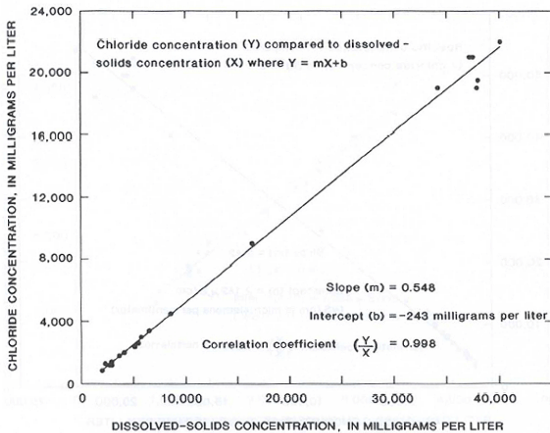
Figure 9. Relation between concentrations of dissolved solids and chloride for 19 water samples from the Floridan aquifer system in southeastern Florida.
