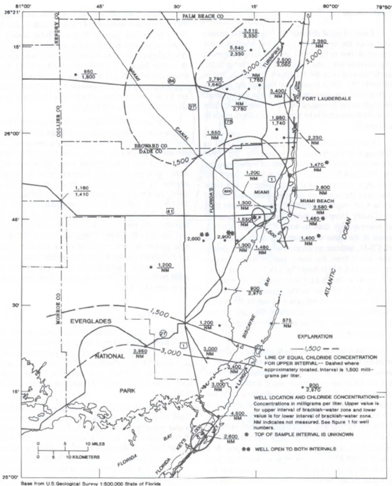
Figure 16. Chloride concentration in ground water from the upper and lower intervals of the brackish-water zone in southeastern Florida. Boundary used between the upper and lower interval: is 200 to 300 feet below the top of the rocks of Eocene age.
