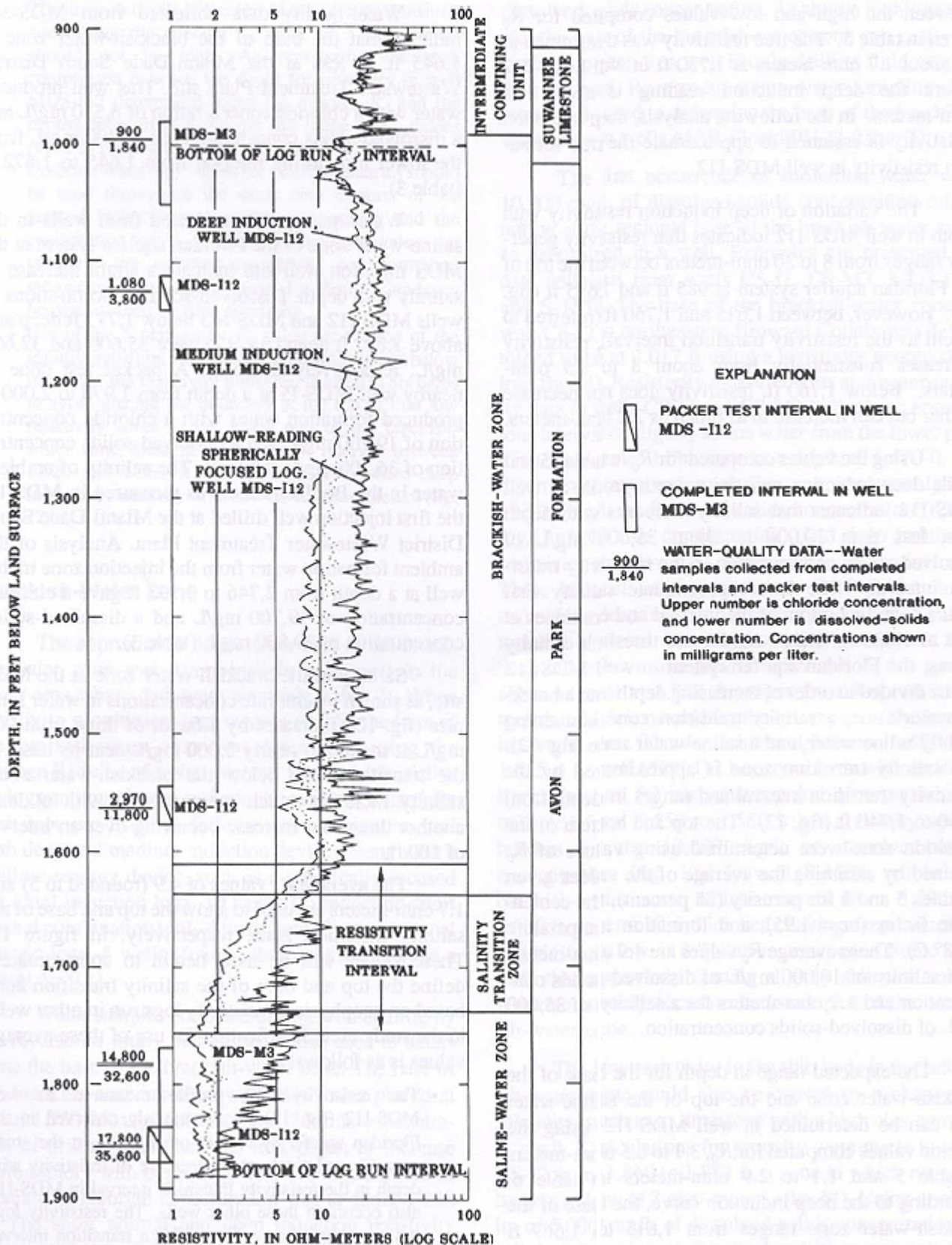
Figure 12. Water-quality data, resistivity geophysical log, salinity zones, and geologic units for twin wells MDS-I12 and MDS-M3 near Biscayne Bay in southeastern Dade County.
