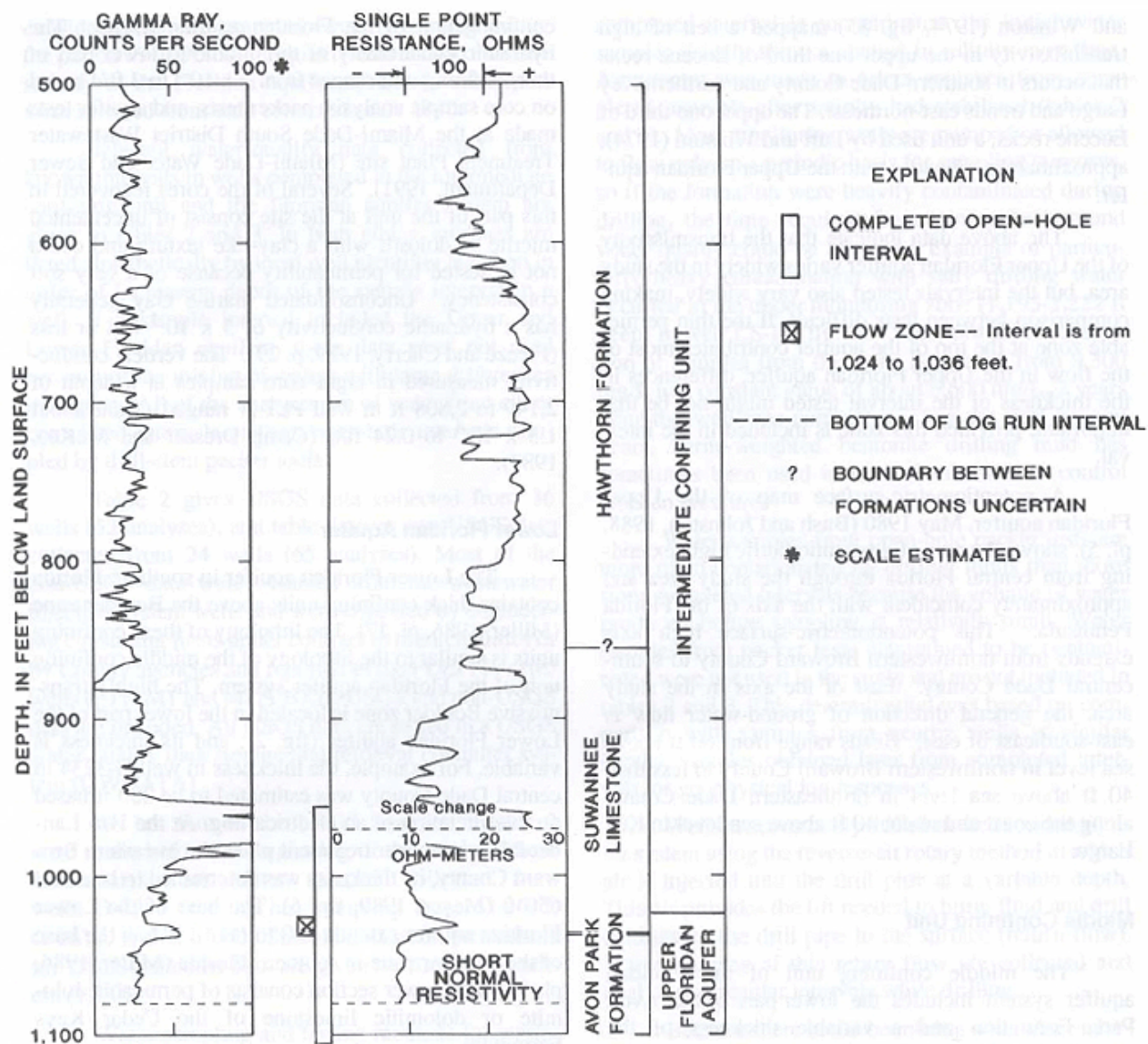
Figure 7. Geophysical logs of well G-3061 showing location of flow zone at the top of the Upper Floridan aquifer and geologic and hydrogeologic units in northeastern Dade County. Flow zone determined from flowmeter log.
