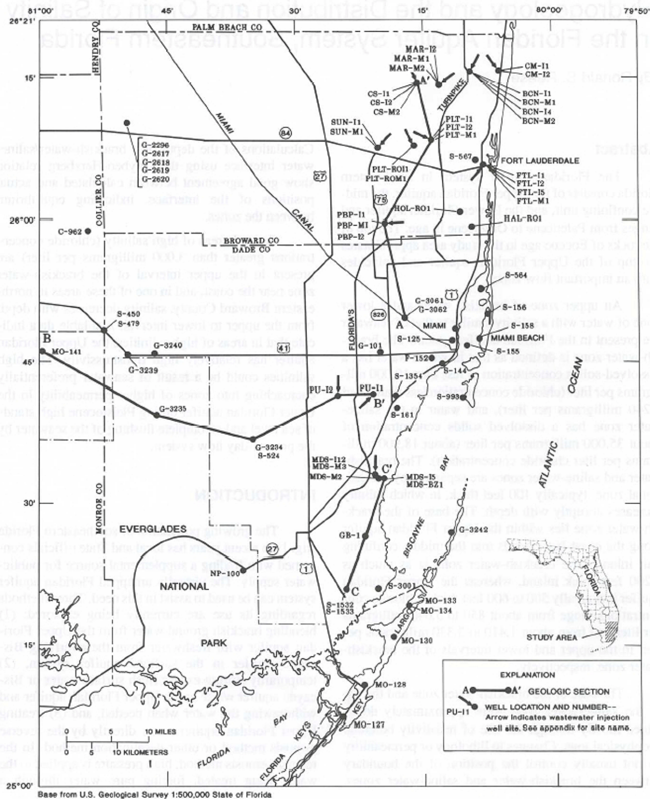
Figure 1. Location of the study area, wells penetrating the Floridan aquifer system used in the study, and geologic section lines.
