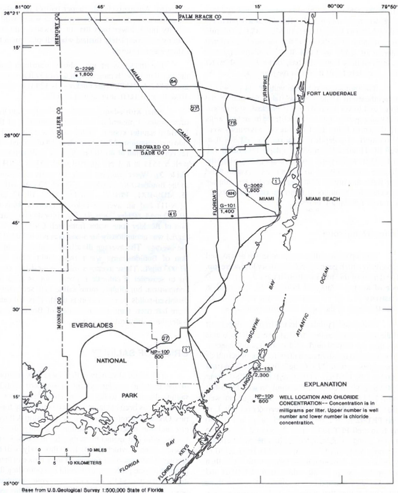
Figure 17. Chloride concentration in ground water from the lower part of the intermediate confining unit in southeastern Florida.
