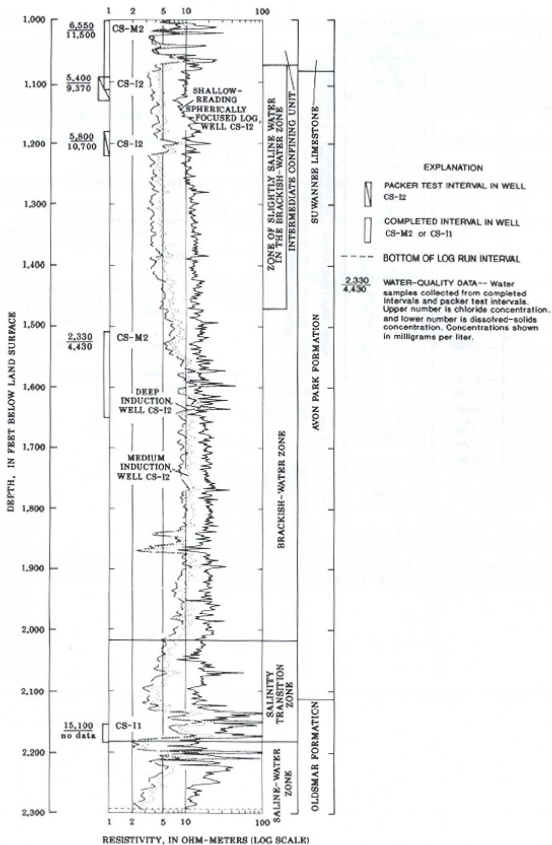
Figure 14. Water-quality data, resistivity geophysical log, salinity zones, and geologic units for twin wells CS-I2 and CS-M2 in northeastern Broward County. One water-quality analysis from well CS-I1, 750 feet south of well CS-I2, is also included in the data.
