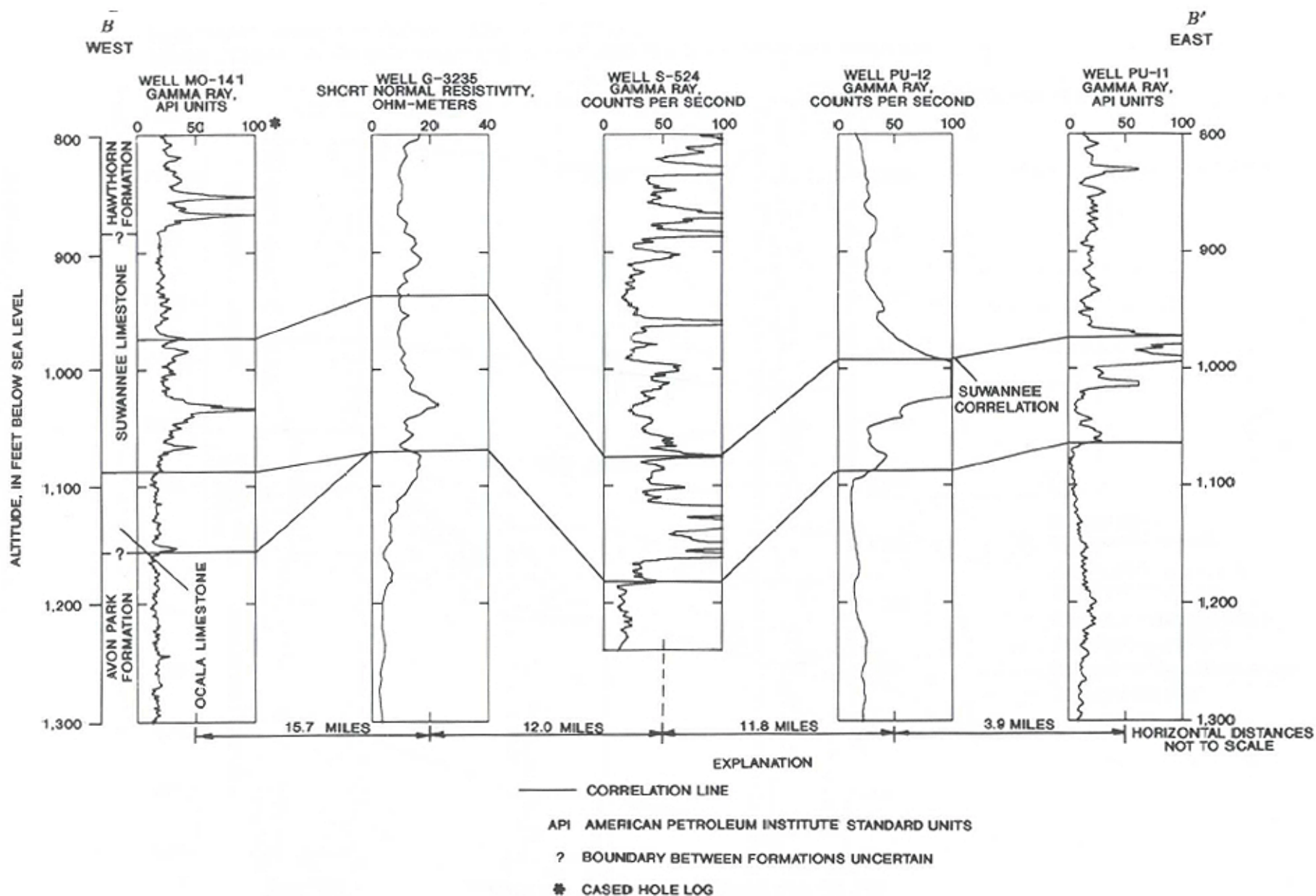
Figure 4. Generalized geologic section B-B' showing correlations in and at the base of the Suwannee Limestone in eastern Monroe and central Dade Counties. A gamma-ray log was not run on well G-3235 (instead a resistivity log was used). Line of section shown in figure 1.
