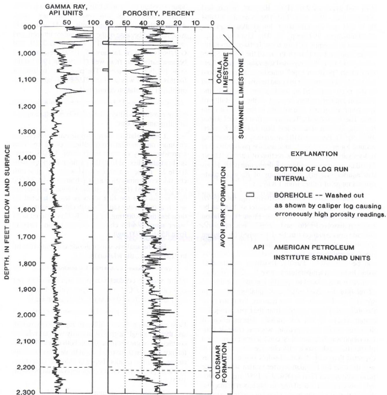
Figure 8. Variations of average porosity with depth derived from a borehole-compensated neutron-density log of well C-962 showing geologic units and a gamma-ray log in eastern Collier County. Porosity is an average of neutron and density responses. Tool was calibrated to a limestone matrix.
