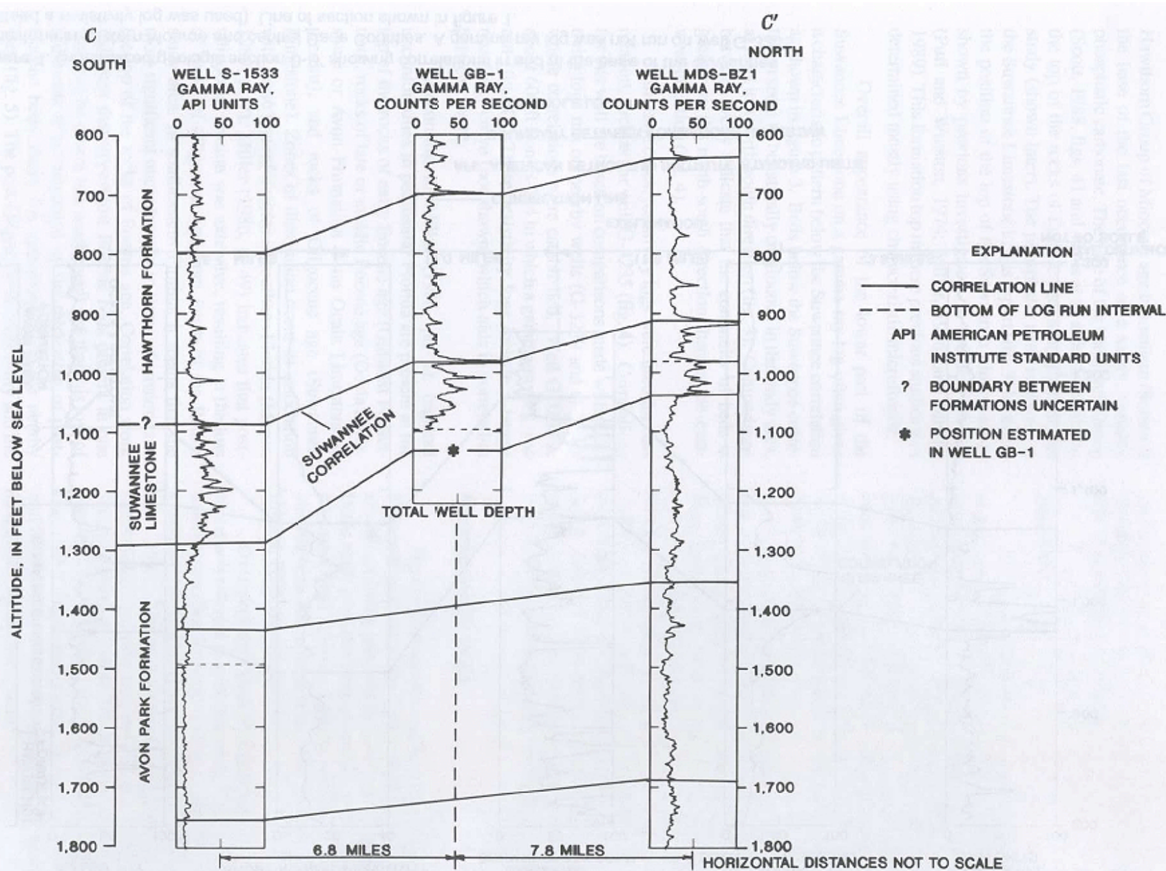
Figure 5. Generalized geologic section C-C' showing thickening of the Suwannee Limestone in southeastern Dade County. Line of section shown in figure 1.
