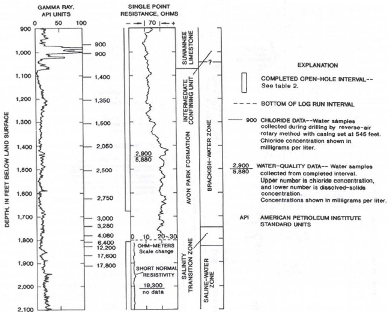
Figure 13. Selected geophysical logs of well PU-11 showing water-quality data collected during drilling by the reverse air rotary method and from completed intervals, geologic units, and salinity zones in eastern Dade County.
