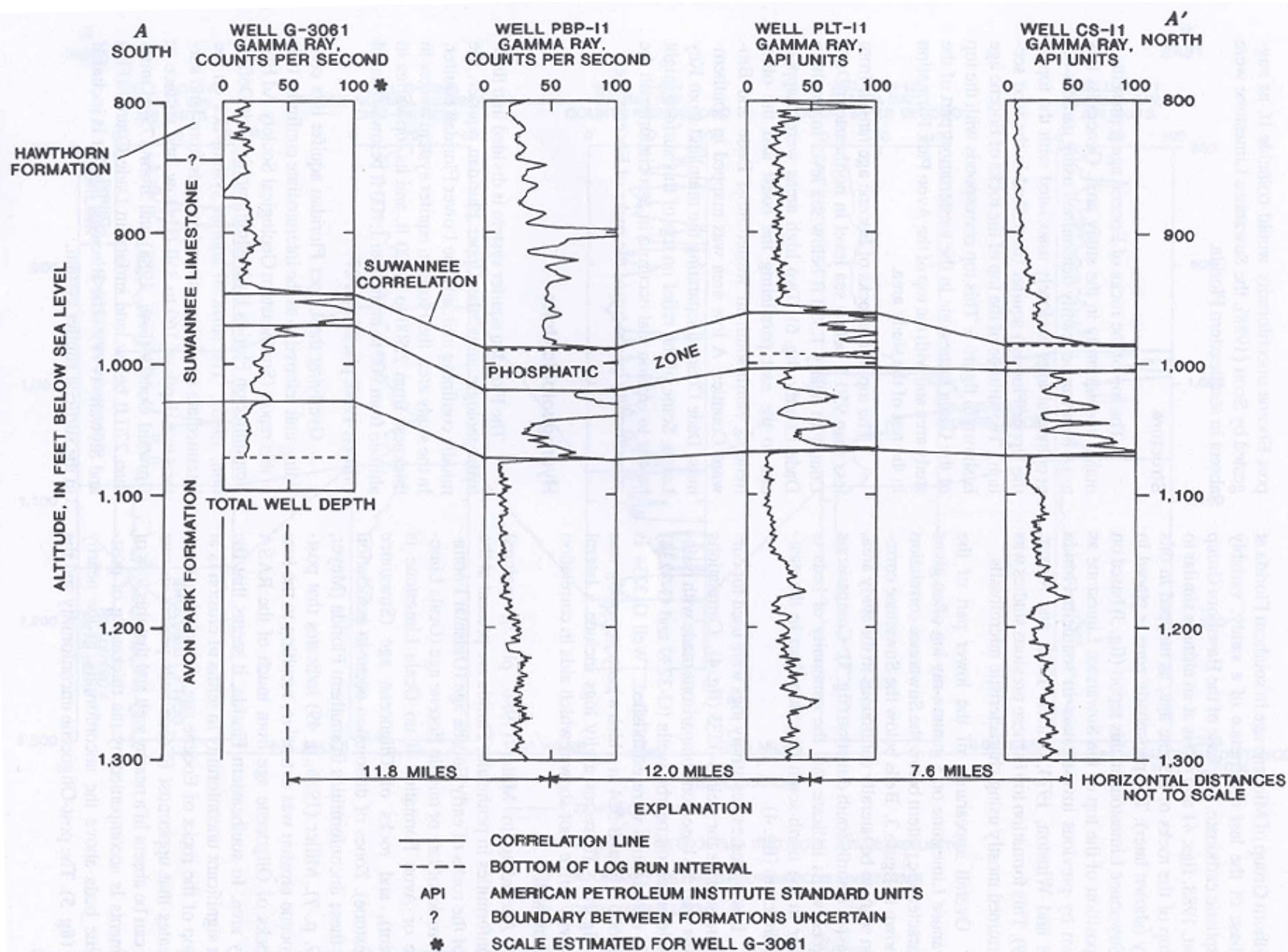
Figure 3. Generalized geologic section A-A' showing correlations in and at the base of the Suwannee Limestone in northern Dade and southern Broward Counties. Line of section shown in figure 1.
