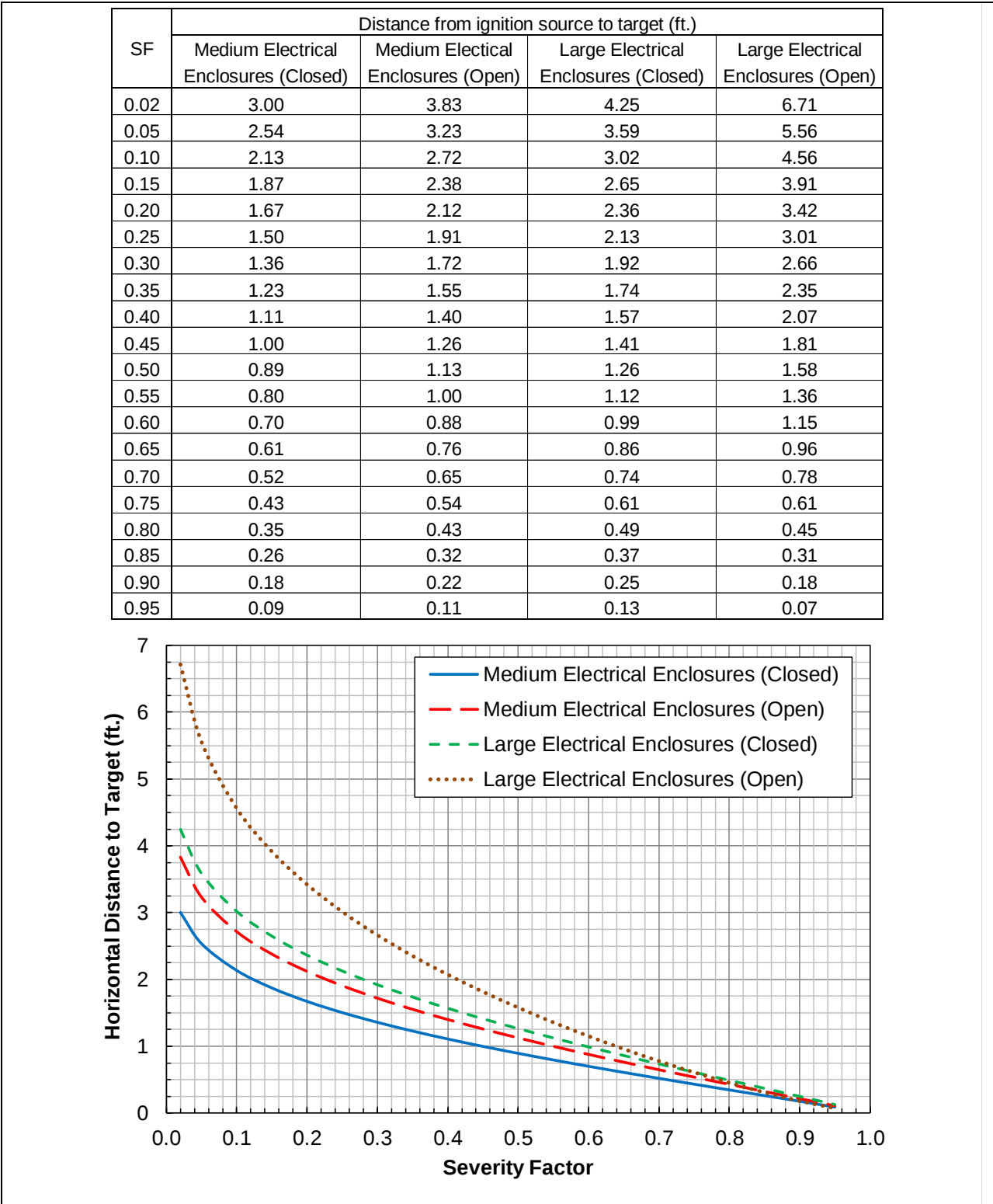
Figure E.08: Severity Factor vs. Radial Target Distance for Electrical Enclosures (Set 2) (TP Cable Targets)
