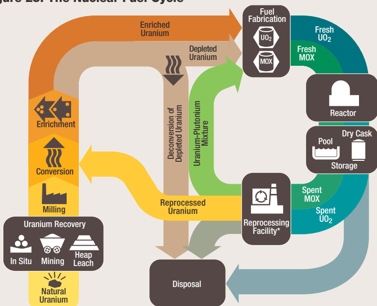
Figure 25. The Nuclear Fuel Cycle
