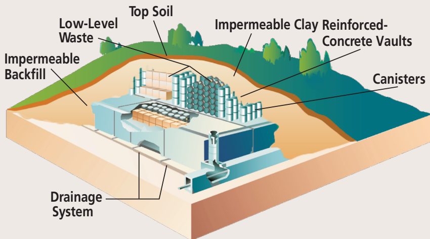
Figure 30. Low-Level Radioactive Waste Disposal
