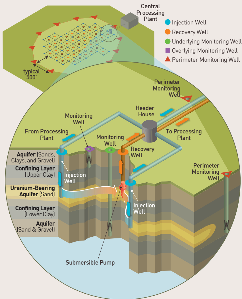
Figure 26. The In Situ Uranium Recovery Process
