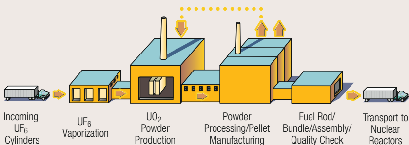
Figure 29. Simplified Fuel Fabrication Process
