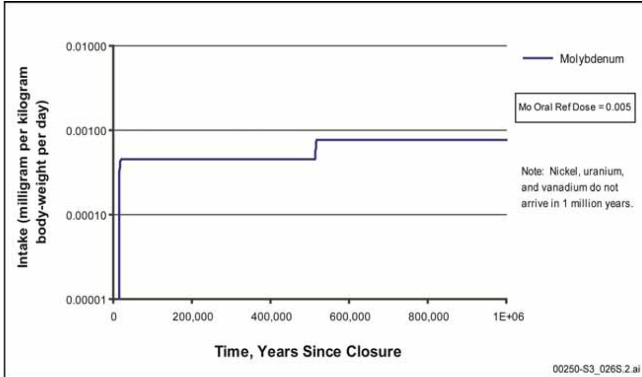
Figure S-12. Molybdenum daily intakes at Furnace Creek springs, no-pumping, wetter climate.
