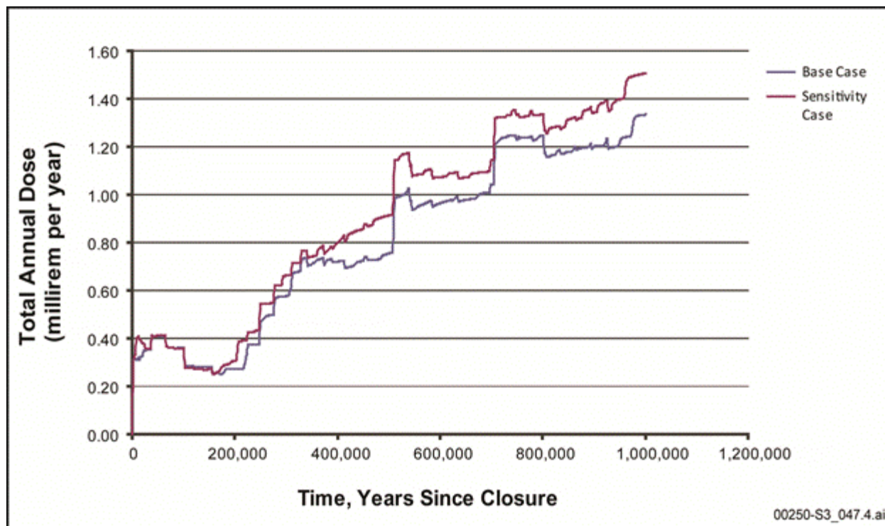
Figure B-24. Sensitivity case for the Amargosa Farms area, pumping, wetter climate.
