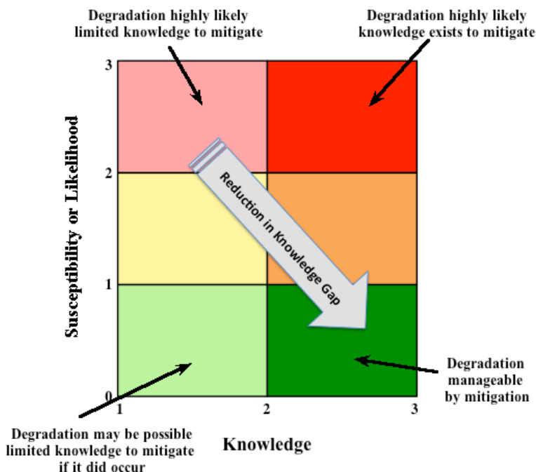
Figure 1.1. Schematic illustrating the combinations of Susceptibility and Knowledge scores suggesting various life management responses.
