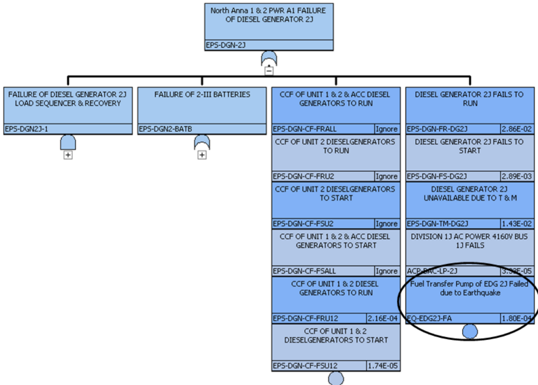
Figure B-10. North Anna, Unit 1 EPS-DGN-2J Fault Tree.
