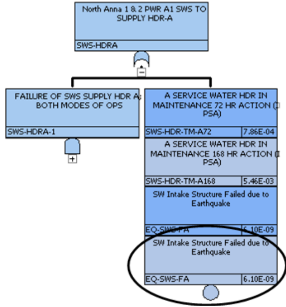
Figure B-11. North Anna, Unit 1 SWS-HDRA Fault Tree.
