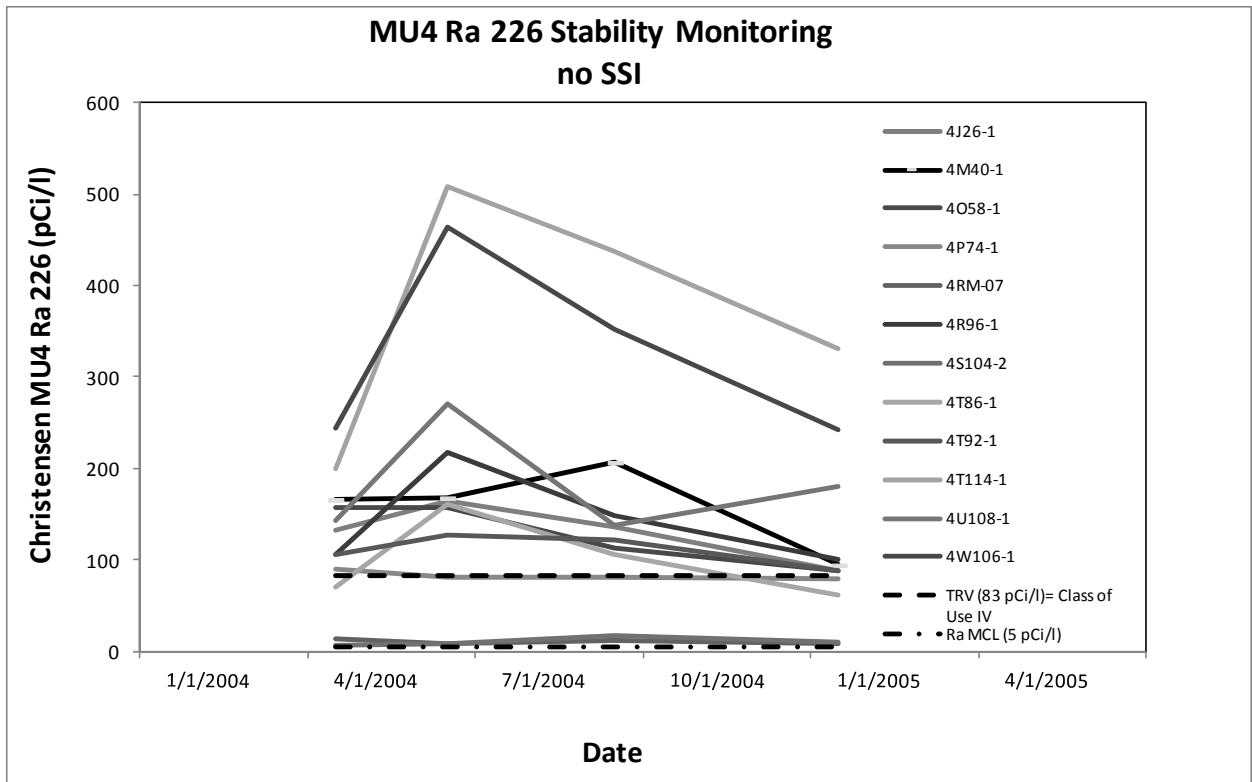
Figure 5c. MU4 Ra 226 Stability Monitoring Trend Analysis
