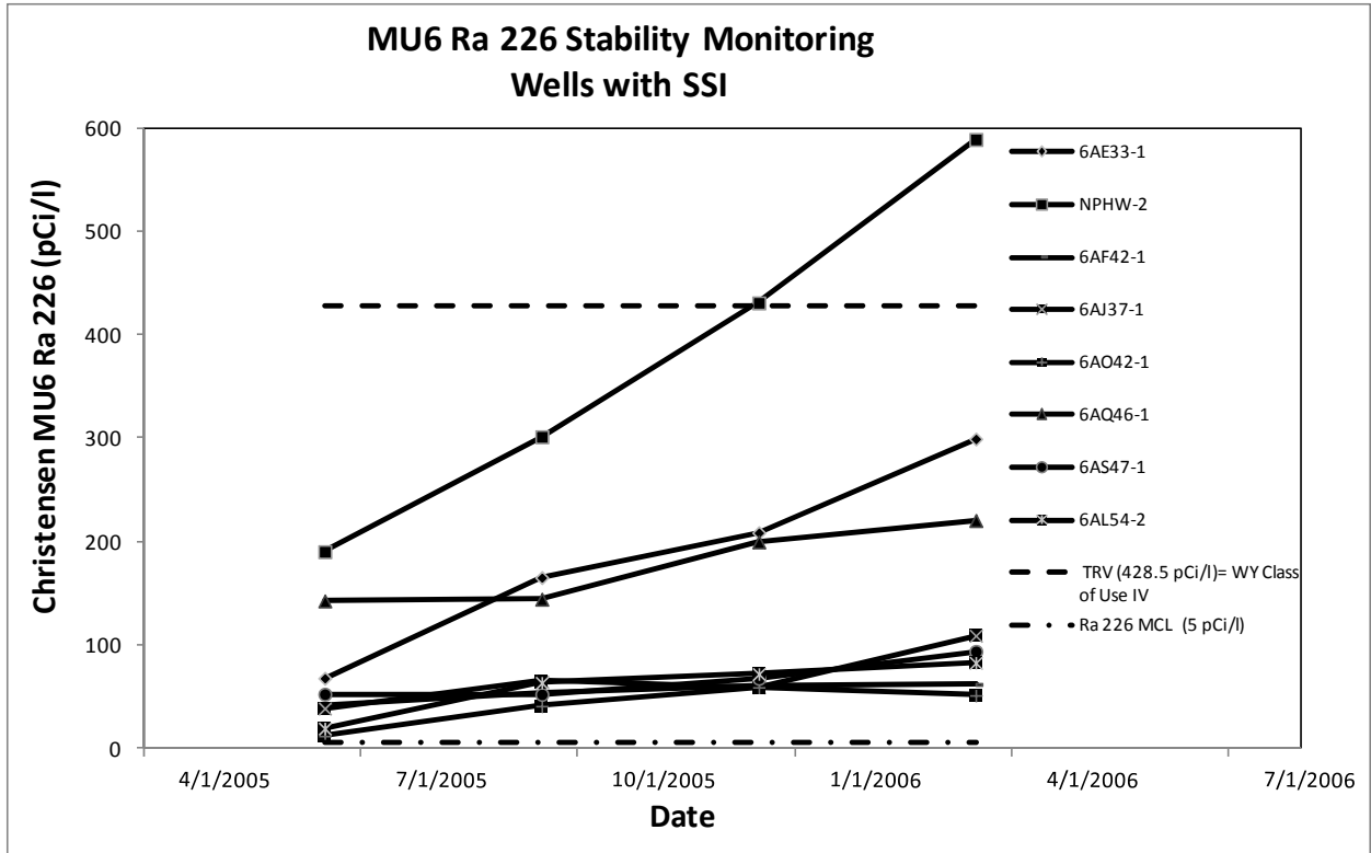
Figure 7c. MU6 Ra 226 Stability Monitoring Trend Analysis
