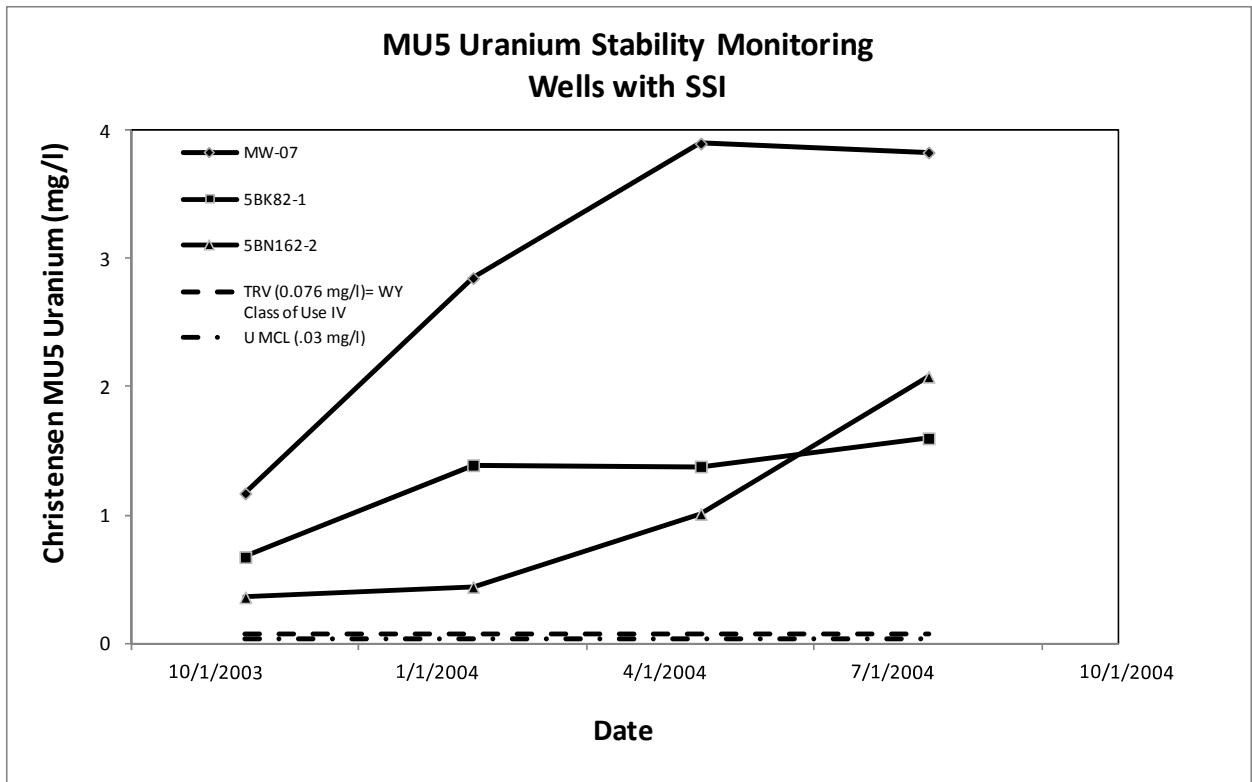
Figure 6b. MU5 Uranium Stability Monitoring Trend Analysis
