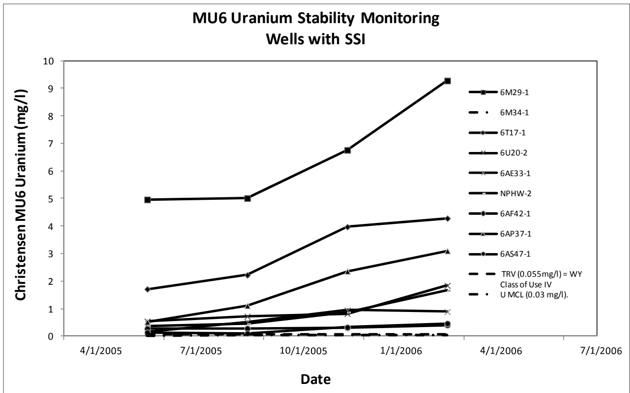
Figure 7b. MU6 Uranium Stability Monitoring Trend Analysis
