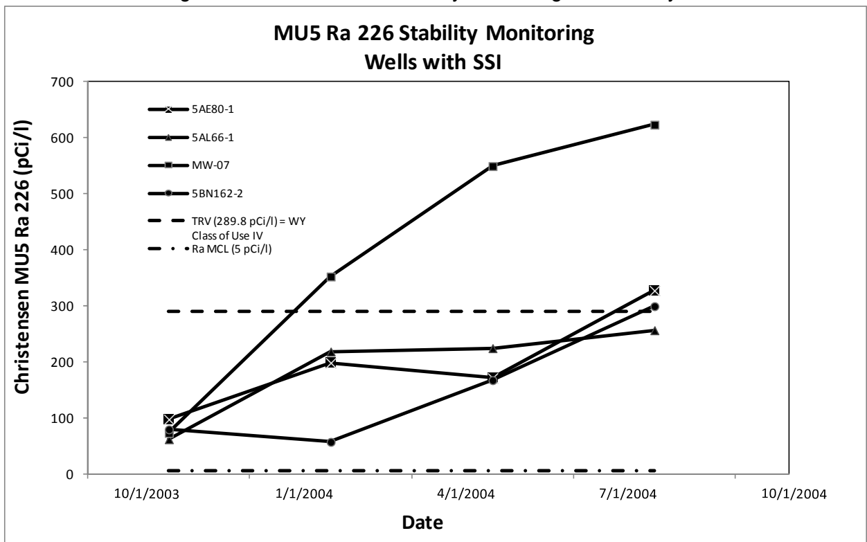
Figure 6c. MU5 Ra 226 Stability Monitoring Trend Analysis
