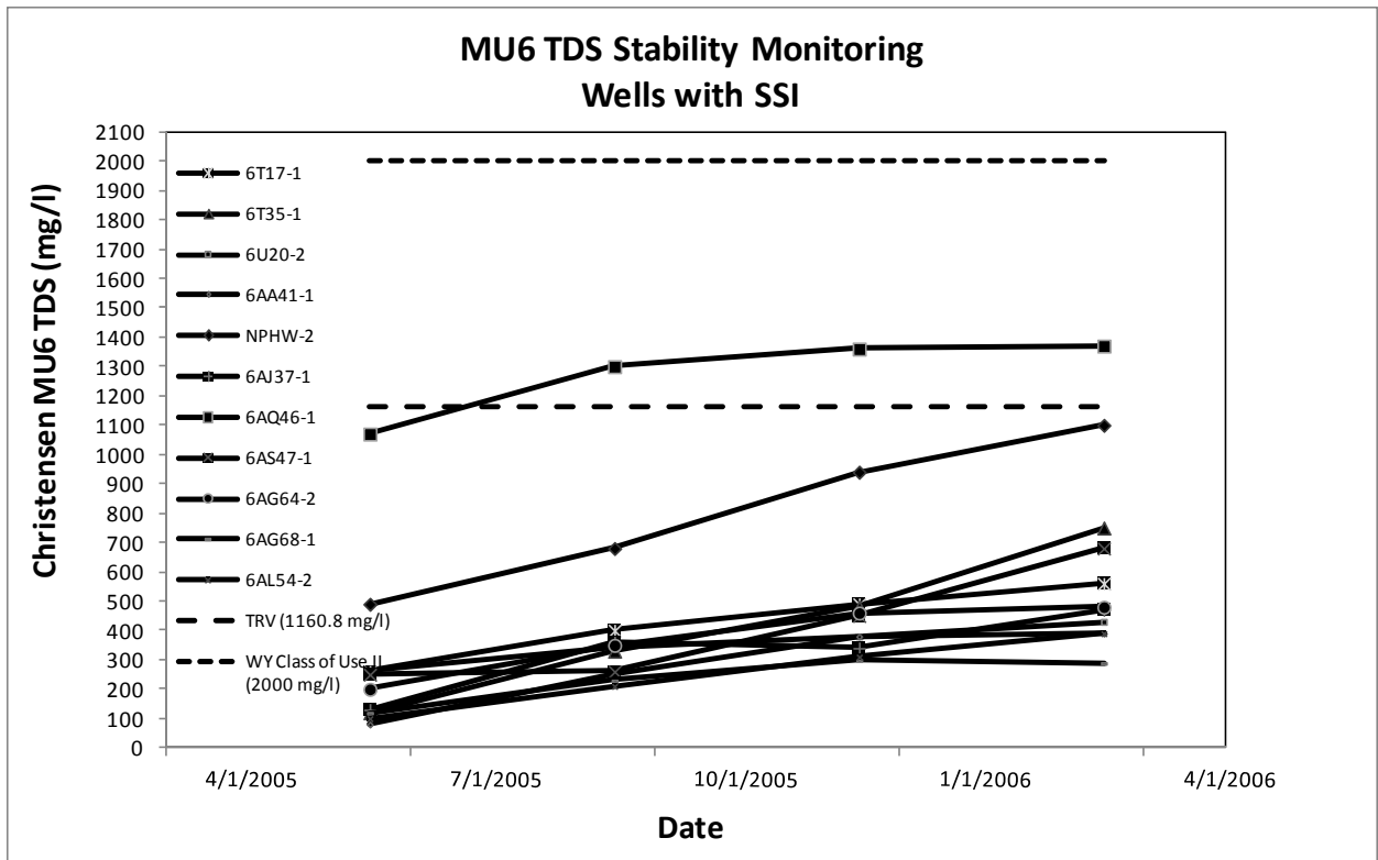
Figure 7a. MU6 TDS Stability Monitoring Trend Analysis
