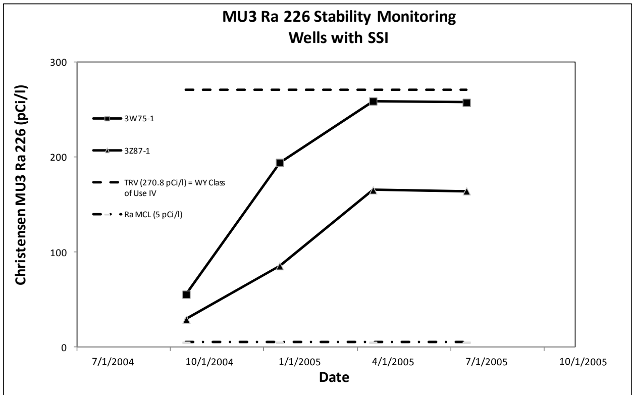
Figure 4c. MU3 Ra 226 Stability Monitoring Trend Analysis
