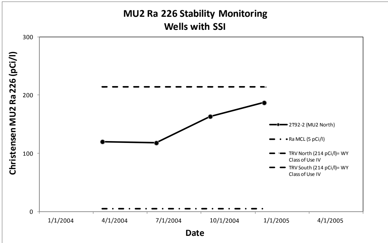
Figure 3c. MU2 North and South Ra 226 Stability Monitoring Trend Analysis
