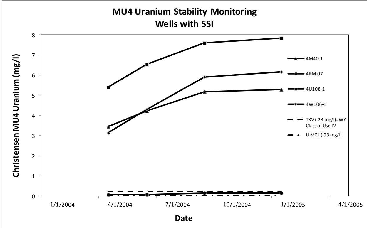
Figure 5b. MU4 Uranium Stability Monitoring Trend Analysis
