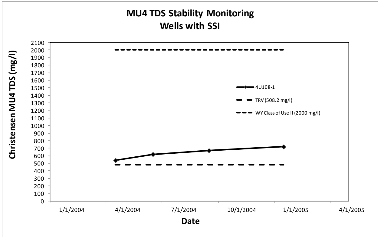
Figure 5a. MU4 TDS Stability Monitoring Trend Analysis
