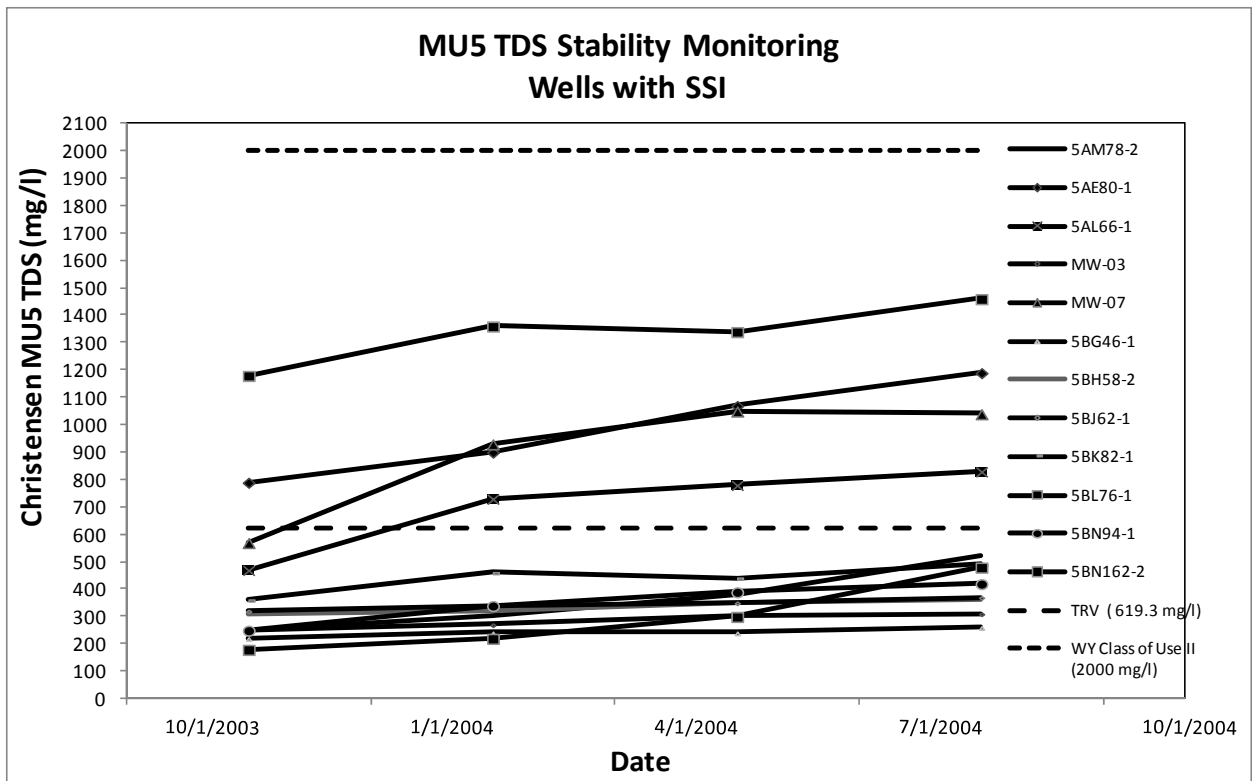
Figure 6a. MU5 TDS Stability Monitoring Trend Analysis
