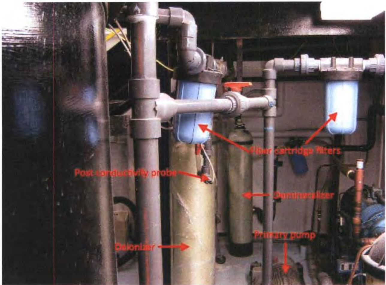
Figure 5.2-1 The UUTR's primary coolant system
