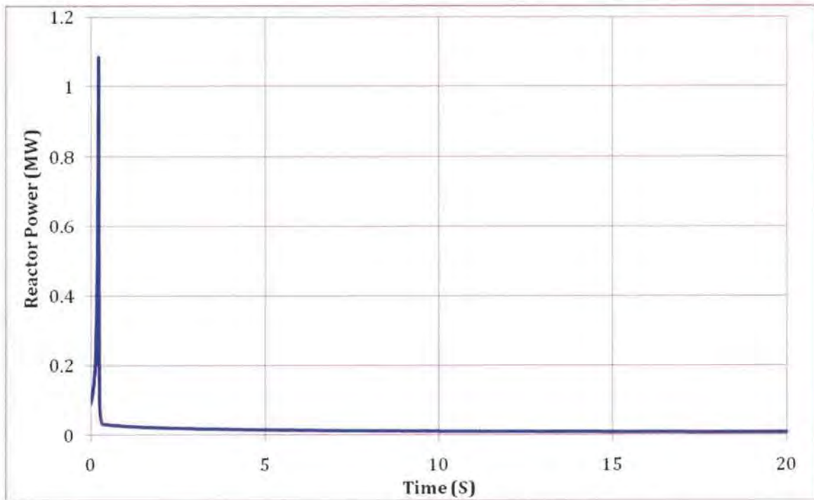
Figure 13.2-5 UUTR reactor power change versus reactor time for $1.2 reactivity insertion accident
