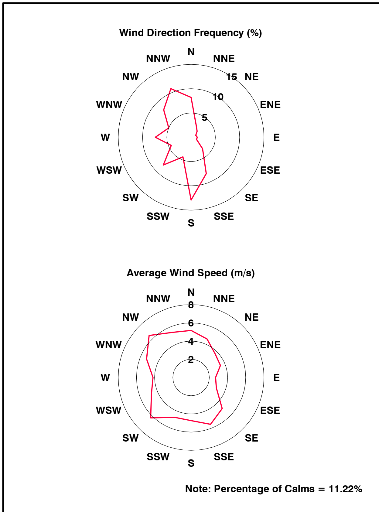
Figure 3. Wind Rose for Gillette - 2009
