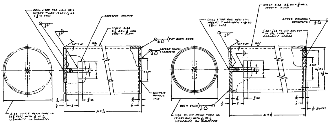
Figure 10.3: Beam Tube
