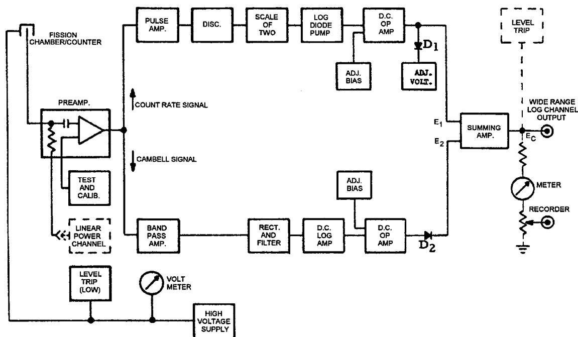
Figure 7.8: Wide Range Log Power Channel Block Diagram
