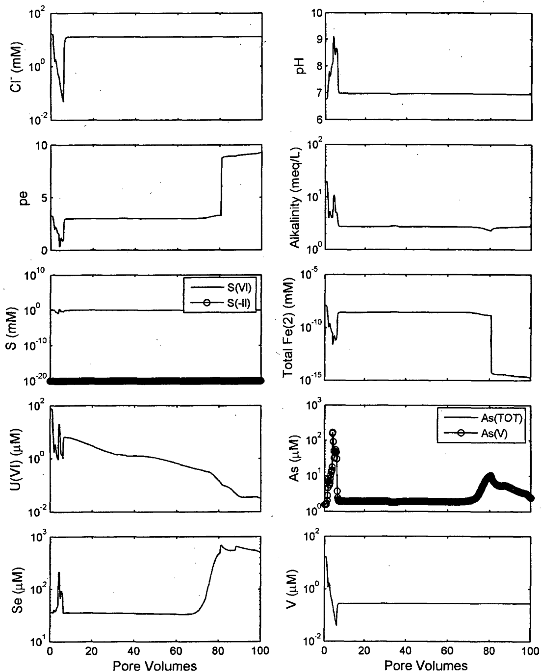
Figure 35. Simulation 18 results. Consideration of the effect of an increase in adsorption site density by a factor of 100. Oxalic influent groundwater. Calcite, goethite, and elemental Se (50 ppm) initially present. 265 mg/L of \text{H}_2\text{S(g)} added to the influent water during pore volumes 3.0 to 3.6. Pyrite and uraninite precipitation not allowed. Amorphous \text{FeS} and \text{UO}_2 precipitation allowed. Mass transfer coefficient = 10. Total sulfide \leq 1 \times 10^{-20} M in plot.
