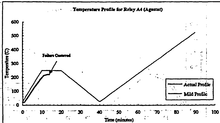
Figure A-4 SCETCH temperature exposure for relay A4
