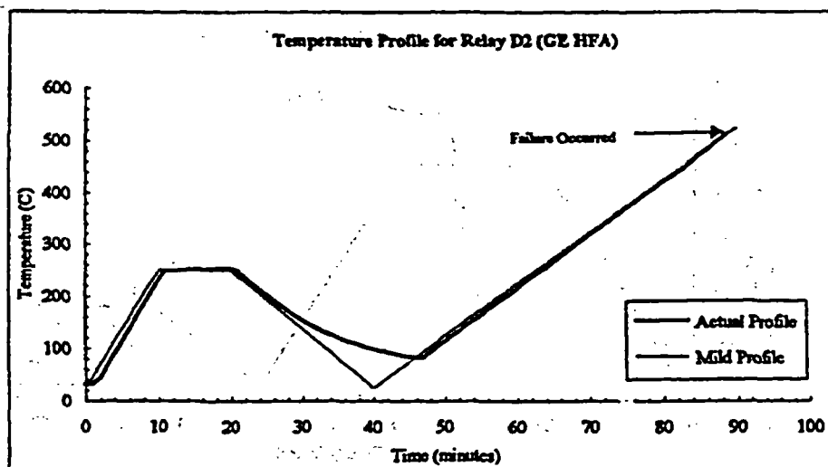
Figure A-16 SCETCH temperature exposure for relay D2
