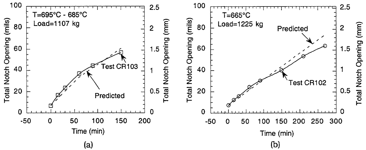
Fig. 11. Experimentally measured and predicted variation of total notch opening with time for specimens with two symmetrical 45° circumferential notches loaded at (a) 1107 kg (2440 lb) and (b) 1225 kg (2700 lb).
