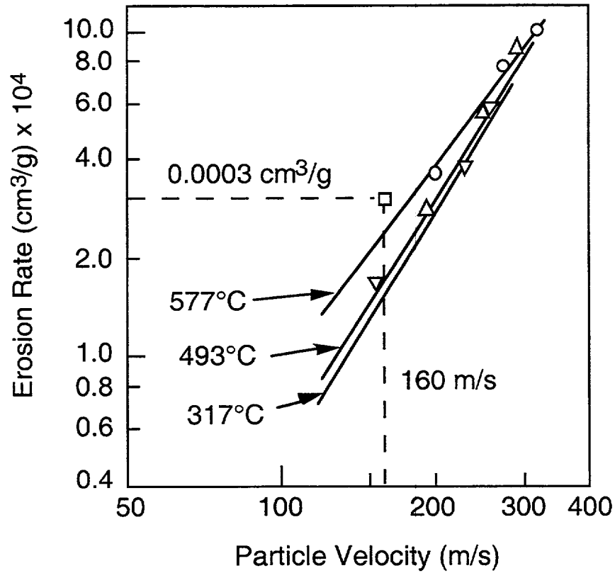
Fig. 1. Erosion rate vs. particle velocity for various temperatures (particle size = 71.5 \mu\text{m} , impingement angle = 30^\circ ); \nabla = 317^\circ\text{C} ( 700^\circ\text{F} ), \Delta = 493^\circ\text{C} ( 920^\circ\text{F} ), \circ = 577^\circ\text{C} ( 1070^\circ\text{F} ). Extrapolated erosion rate for 700^\circ\text{C} ( 1292^\circ\text{F} ) at 160 m/s (520 ft/s) is indicated by the square symbol (figure adapted from Tabakoff and Vittal 22 ).
