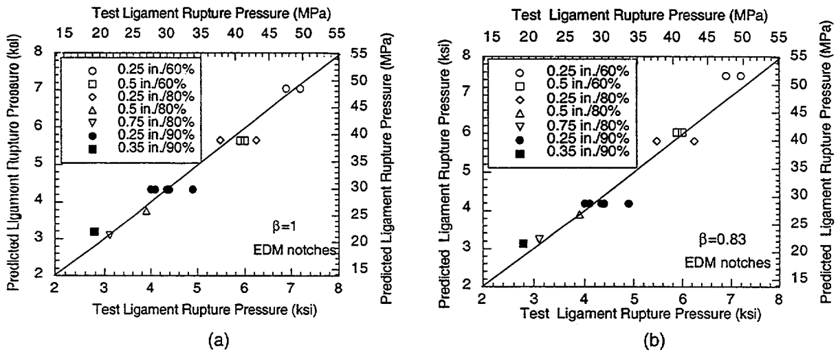
Figure 6. Observed vs. predicted ligament rupture pressures for tubes with EDM notches using (a) k = 0.55 and \beta = 1 and (b) k = 0.595 and \beta = 0.83 .
