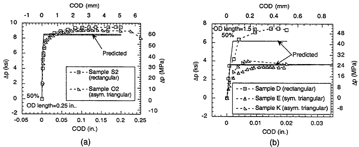
Figure 17. (a) Predicted vs. observed COD for specimens with rectangular and triangular notches with average depth 50% and with OD lengths (a) 6 mm [0.25 in.] and (b) 38 mm [1.5 in.].
