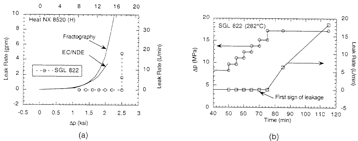
Figure 49. (a) Predicted and measured pressure vs. leak rate plots for specimen SGL-822 conducted at 282°C and (b) pressure and leak rate variation observed during test SGL-822.
