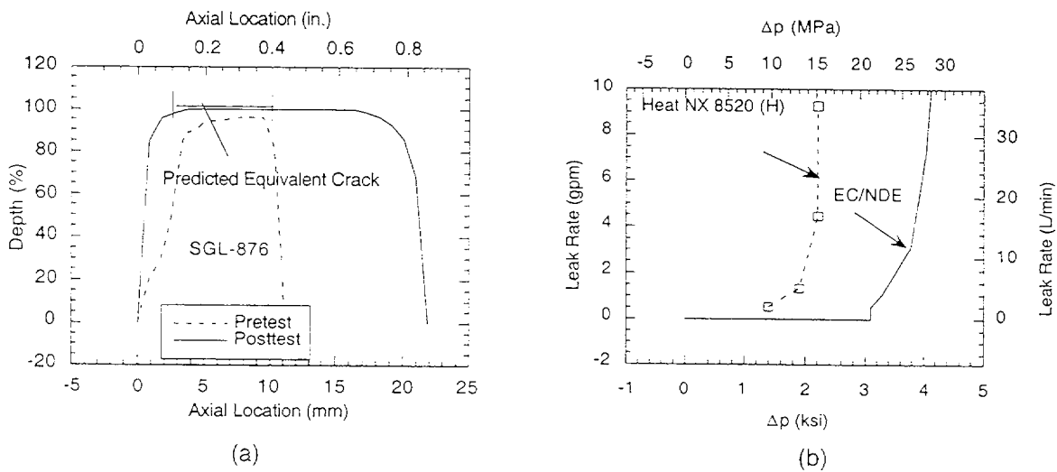
Figure 50. (a) Pretest and posttest (after room-temperature testing) EC/NDE profile of SCC flaw in specimen SGL-876 and (b) observed vs. predicted leak rate curve based on EC/NDE depth profile.
