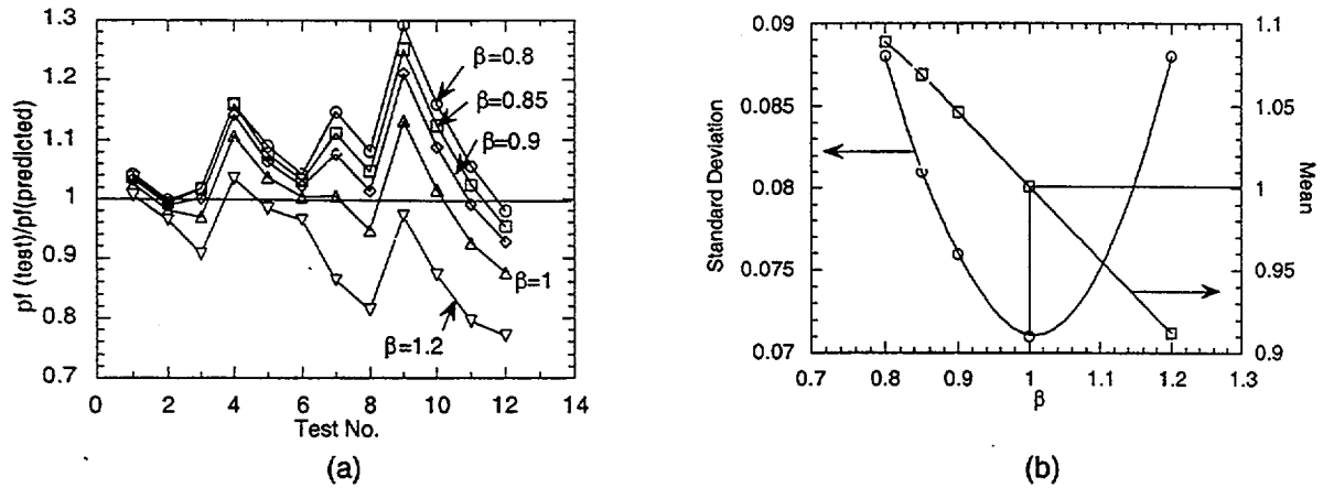
Figure 5. (a) Variation of observed failure pressures divided by predicted failure pressures corresponding to various values of \beta for the ANL tests and (b) variation of the mean and standard deviation of the observed failure pressure divided by predicted failure pressure with \beta .
