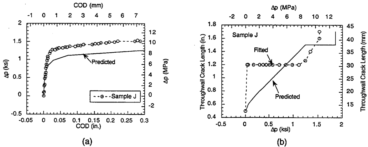
Figure 16. (a) Predicted vs. observed COD and (b) fitted TW crack length needed to match the measured COD vs. predicted TW crack length for specimen J.
