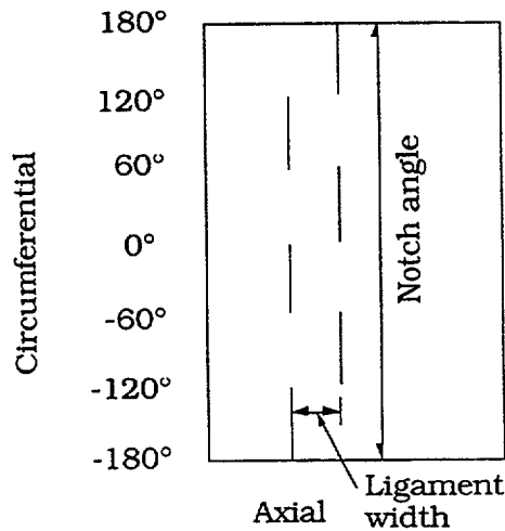
Type 8 specimen
