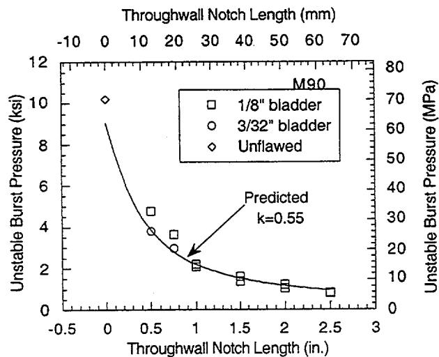
Figure 2. Predicted vs. observed variation of unstable burst pressure with notch length of Heat M90 tubes with TW axial EDM notches.
