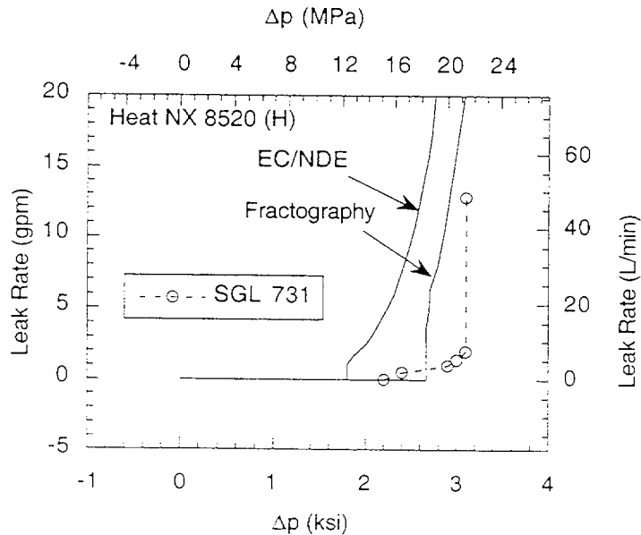
Figure 47. Predicted and measured pressure vs. leak rate plots for SGL-731.
