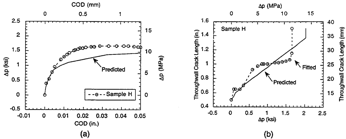
Figure 15. (a) Predicted vs. observed COD and (b) fitted TW crack length needed to match the measured COD vs. predicted TW crack length for specimen H.
