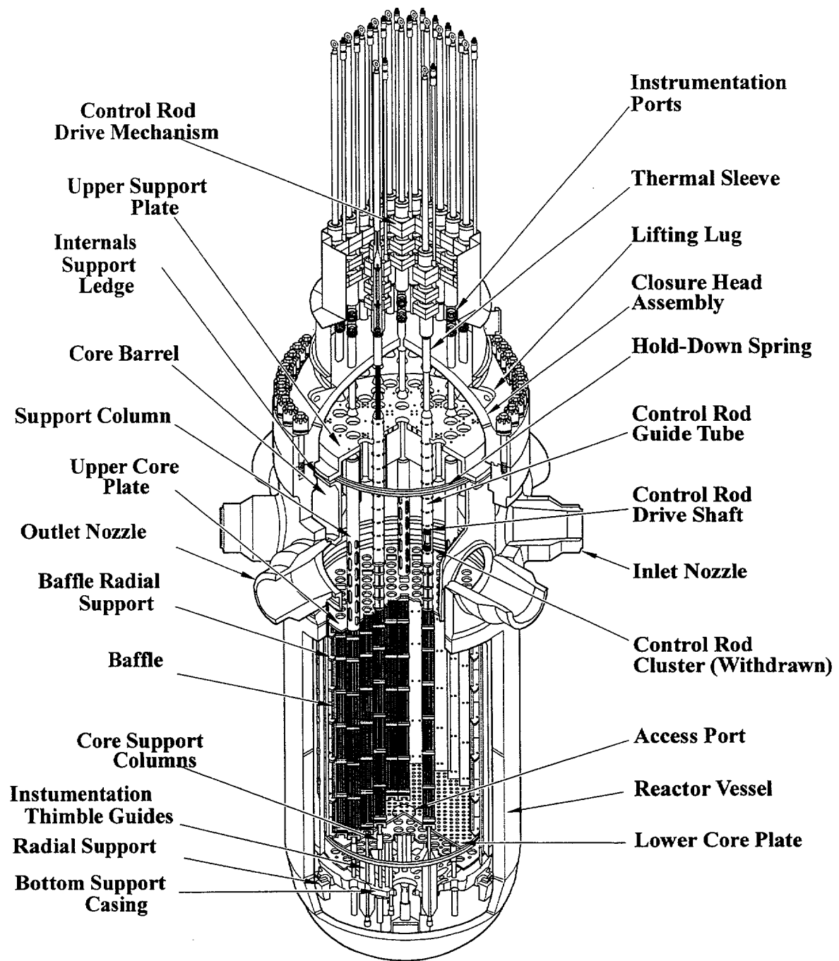
Figure 3.1-9 PWR reactor vessel internals (Westinghouse)
