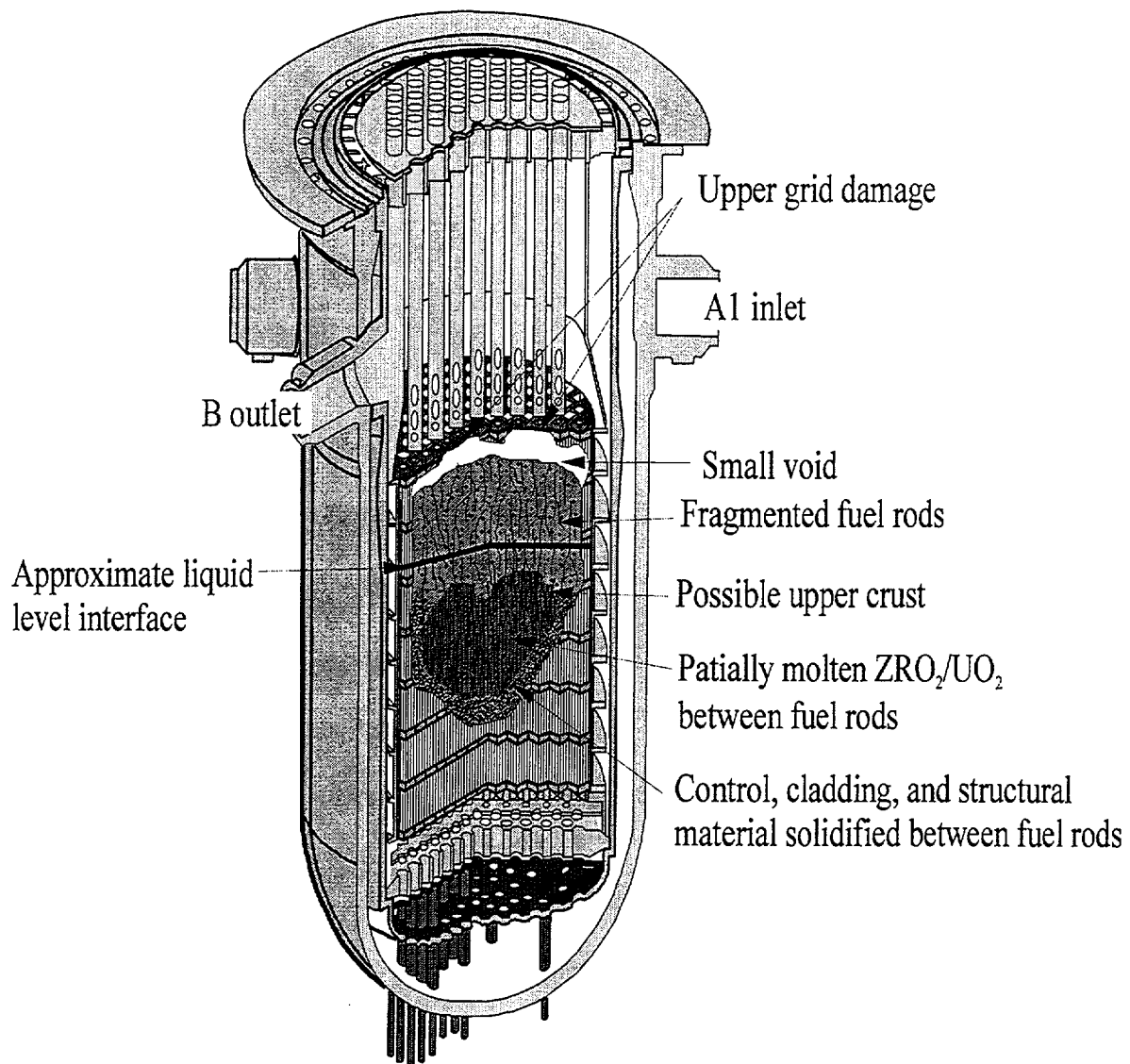
Figure 3.4-6 Hypothesized TMI-2 core configuration between 174 and 180 minutes
