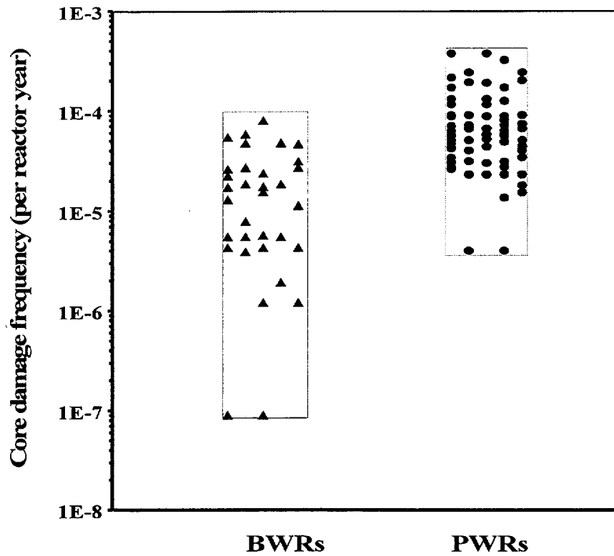
Figure 2.5-10 Reported IPE CDFs for BWRs and PWRs
