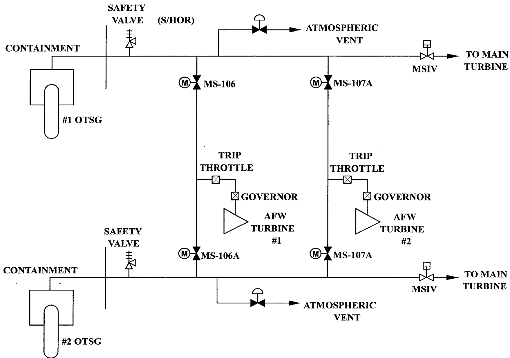
Figure 2A-2 Main steam system
