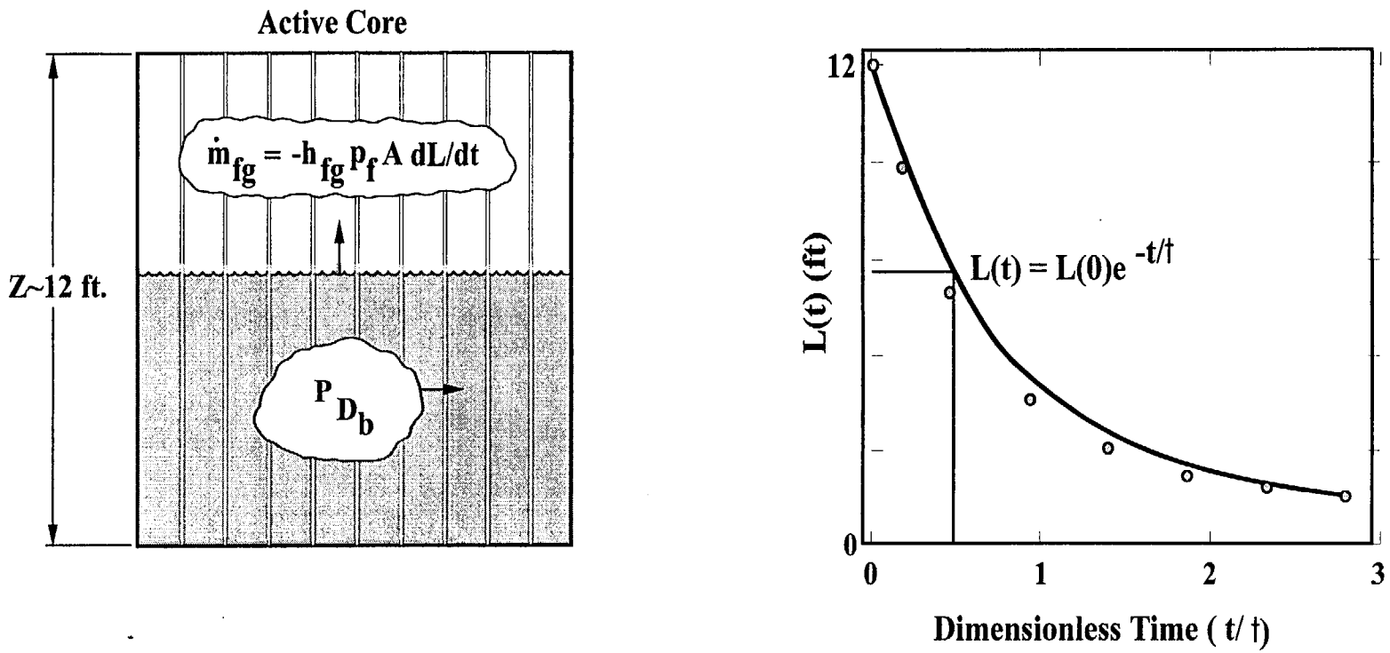
Figure 3.2-1 Exponentially decreasing water level
