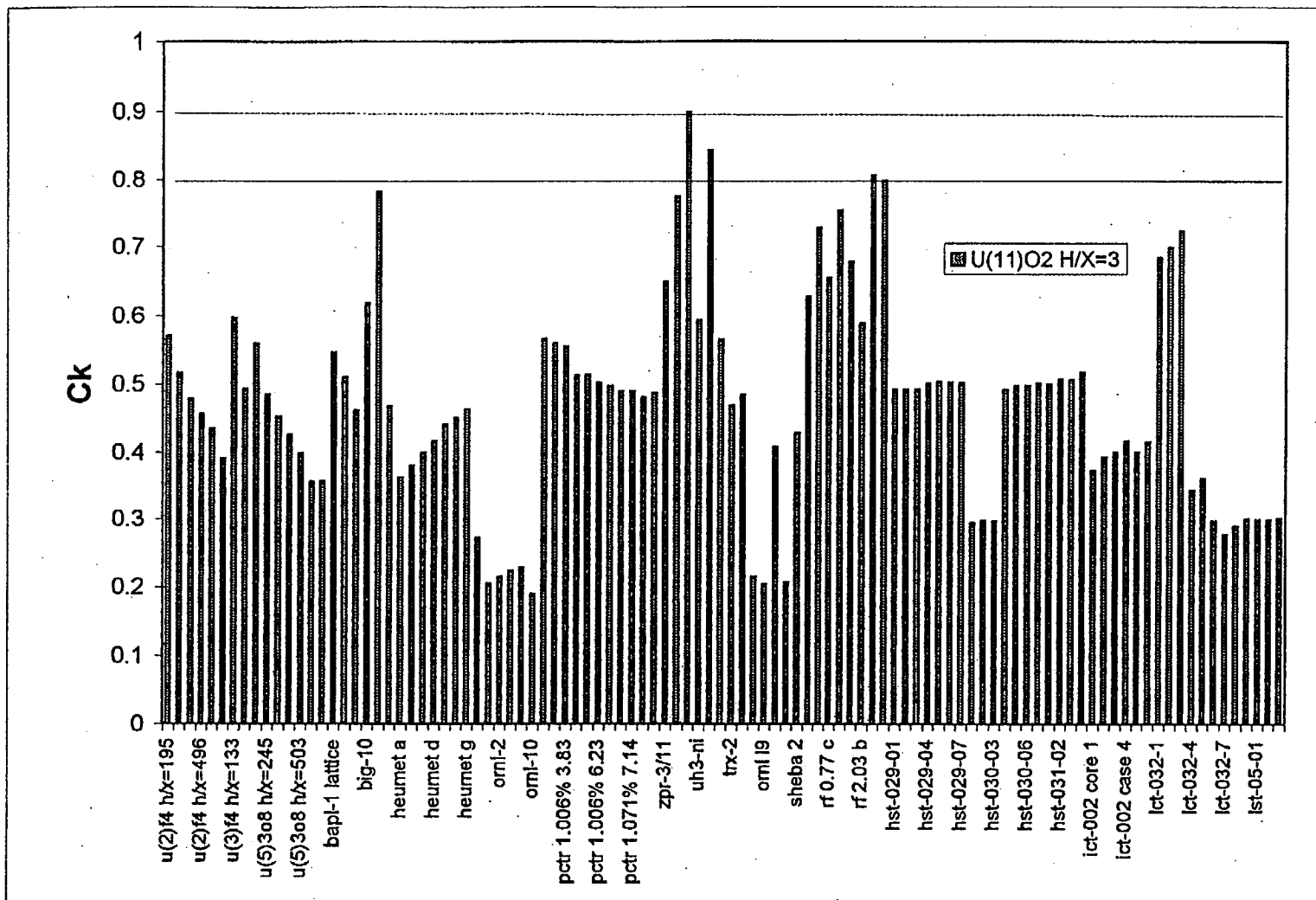
Figure 2 Correlation coefficients, C_k , for U(11)O_2 , H/X = 3 system with 102 benchmark experiments
