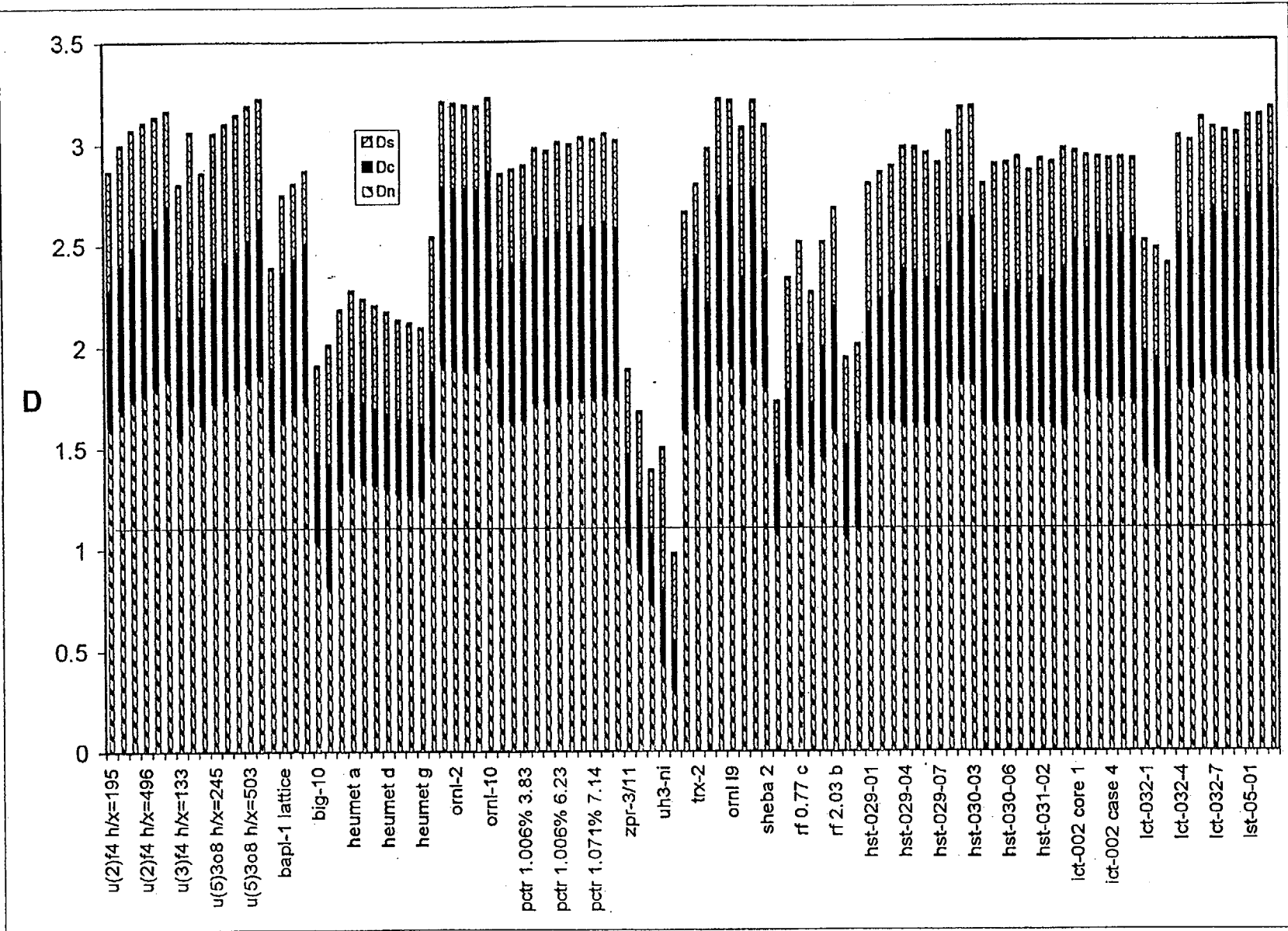
Figure 6 D coefficients for U(11)O_2 , H/X = 3 system with 102 benchmark experiments
